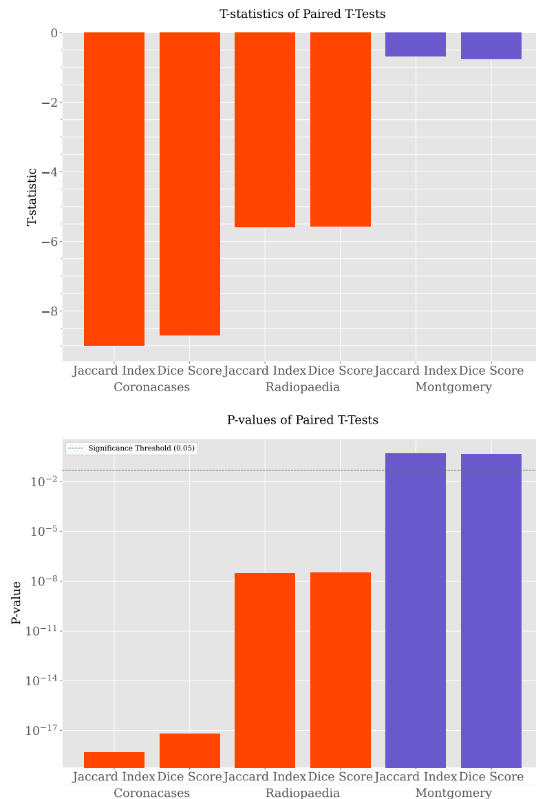
Figure 11. Hypothesis tests.
