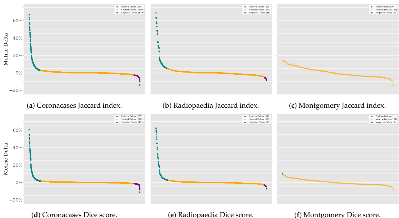
Figure 8. SAM 2 vs. SAM deltas in descending order.
