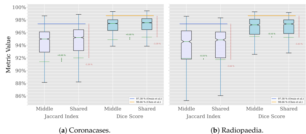
Figure 14. Shared seed video results (Owais et al. [19], Chen et al. [21]).
