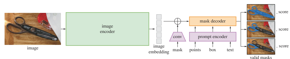
(a) SAM architecture.
