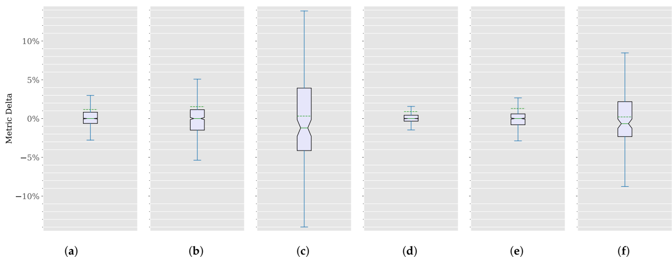
Figure 7. SAM 2 vs. SAM segmentation delta comparison. (a) Coronacases Jaccard index. (b) Radiopaedia Jaccard index. (c) Montgomery Jaccard index. (d) Coronacases Dice score. (e) Radiopaedia Dice score. (f) Montgomery Dice score.
