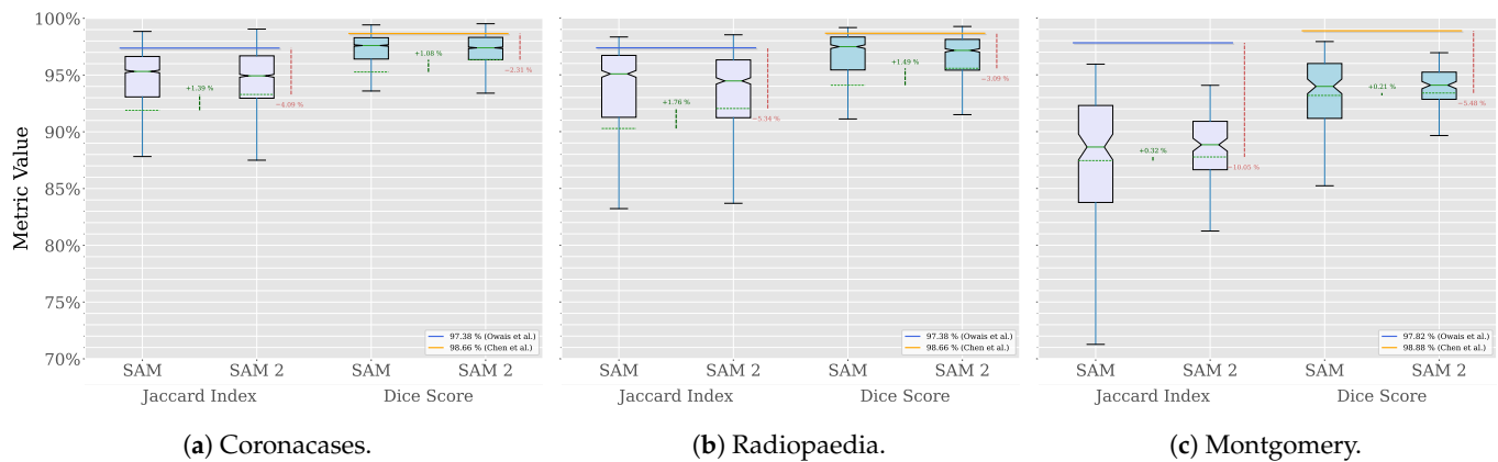
Figure 6. Segmentation comparison (Owais et al. [19], Chen et al. [21]).
