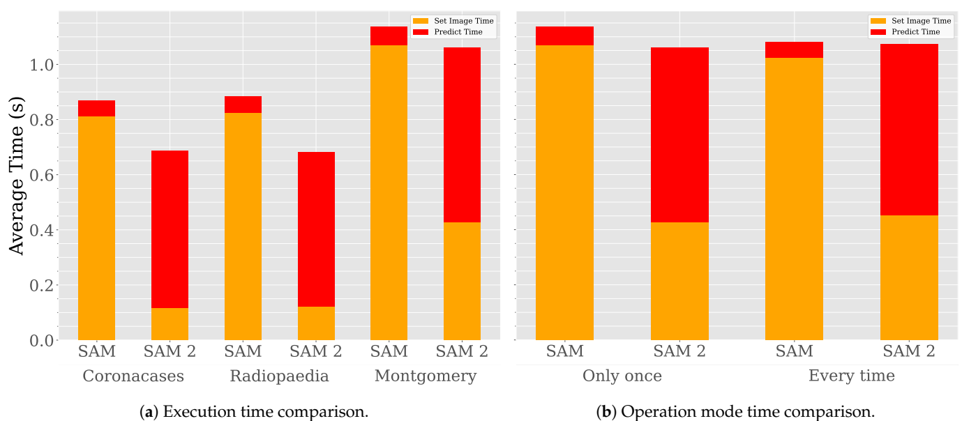
Figure 10. SAM vs SAM 2 time analysis.
