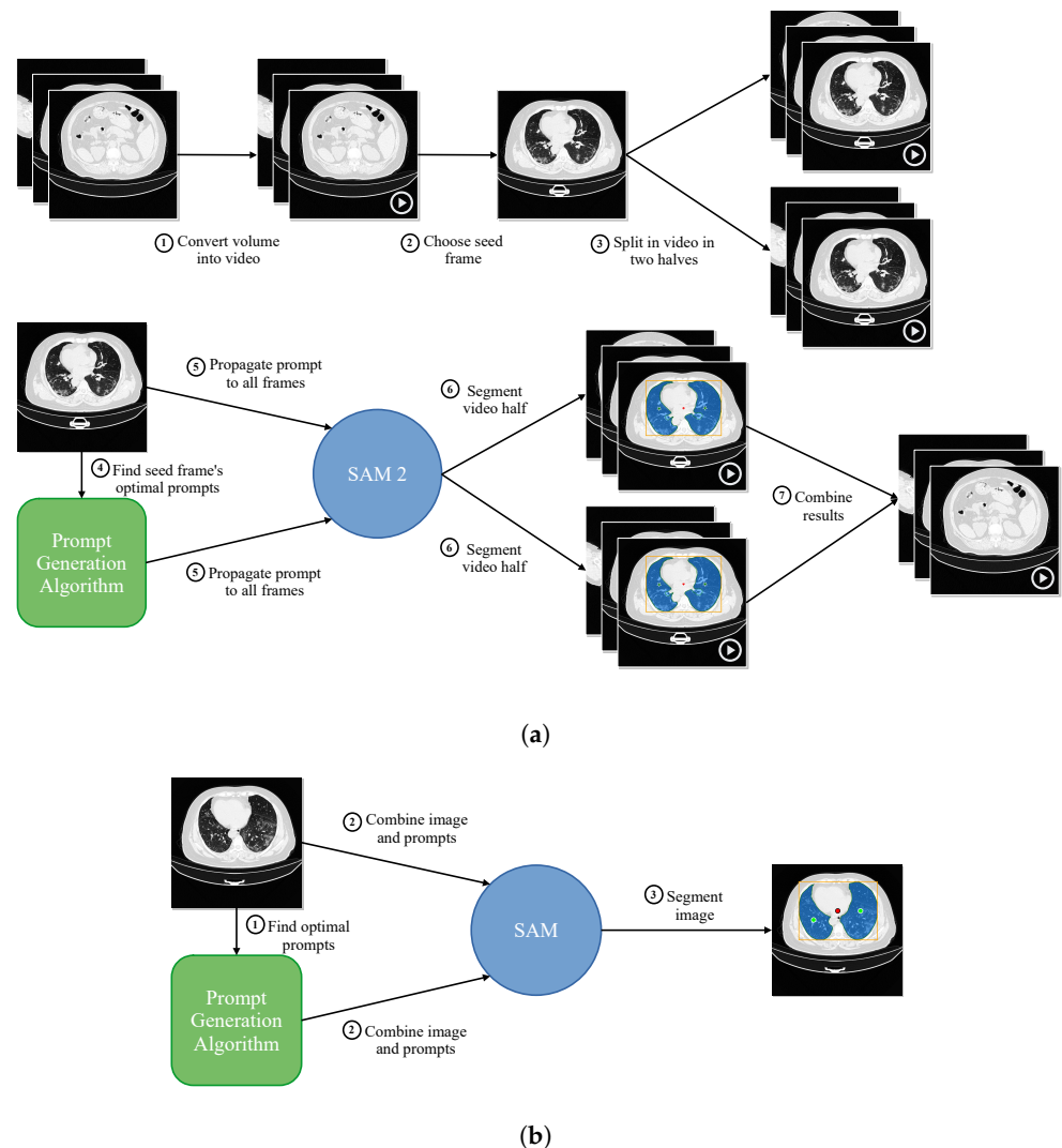
Figure 4. Proposed segmentation process. (a) Proposed segmentation process using SAM 2. (b) Previously proposed segmentation process using SAM [9].
