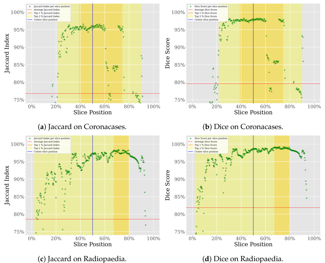
Figure 5. Spatial distribution of segmentation metrics using SAM, with emphasis on the central slice.
