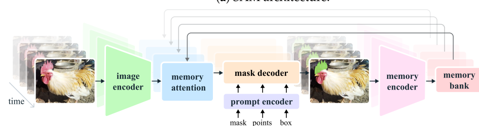
(b) SAM 2 architecture.
