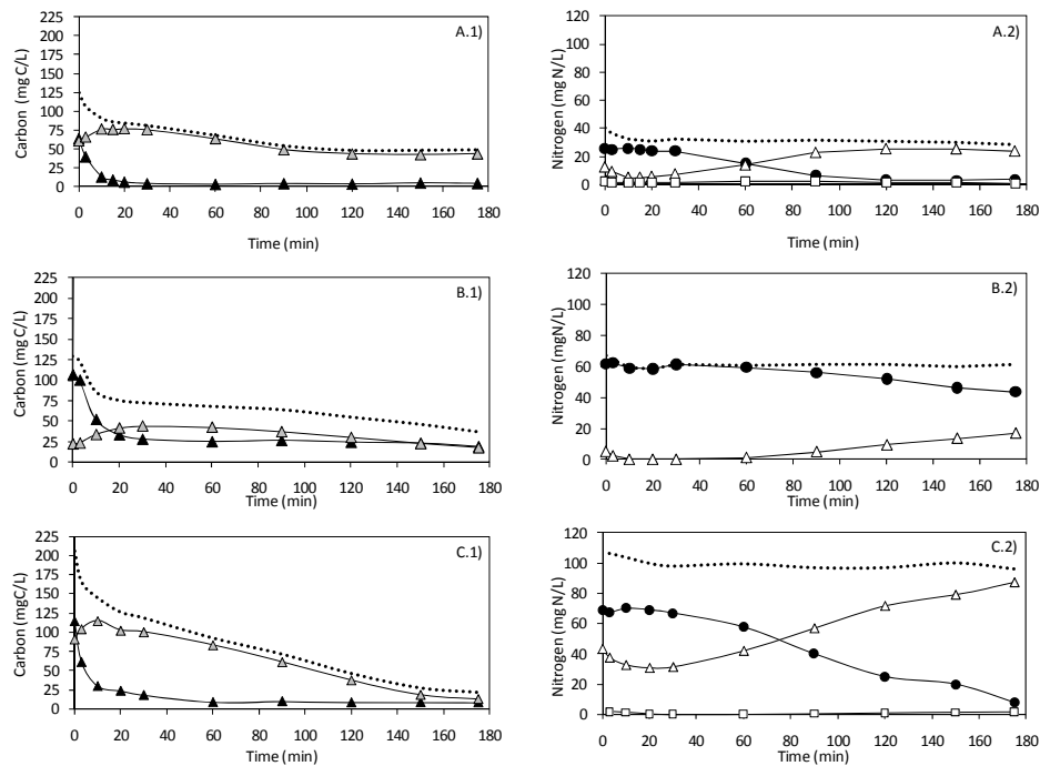
Figure 3.10. 1) IC (▲), TOC (▲) and TC (---). 2) NH 4 + -N (●), NO 2 - -N (△), NO 3 - -N (□) and TN (---) concentrations (mg/L). Cycles performed on operational days A) 148 (S. II), B) 270 (S. IV) and C) 396 (S. V).
