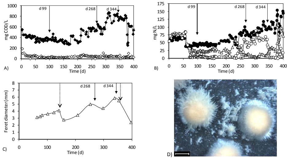
Figure 8.1. Performance of R1 and sampling dates (days 268 and 344) indicated with arrows. A) Organic matter concentration (mg COD/L): \text{COD}_{\text{inf}} (◆), \text{COD}_{\text{eff}} (◇) and B) nitrogen compounds concentrations (mg N/L): \text{NH}_4^+-\text{N}_{\text{inf}} (●), \text{NH}_4^+-\text{N}_{\text{eff}} (○), \text{NO}_2^--\text{N}_{\text{eff}} (△). C) Evolution of the feret diameter (mm) and breakage episodes indicated with dotted arrows. D) Picture of the granules on day 339 with the bar indicating 2 mm.
