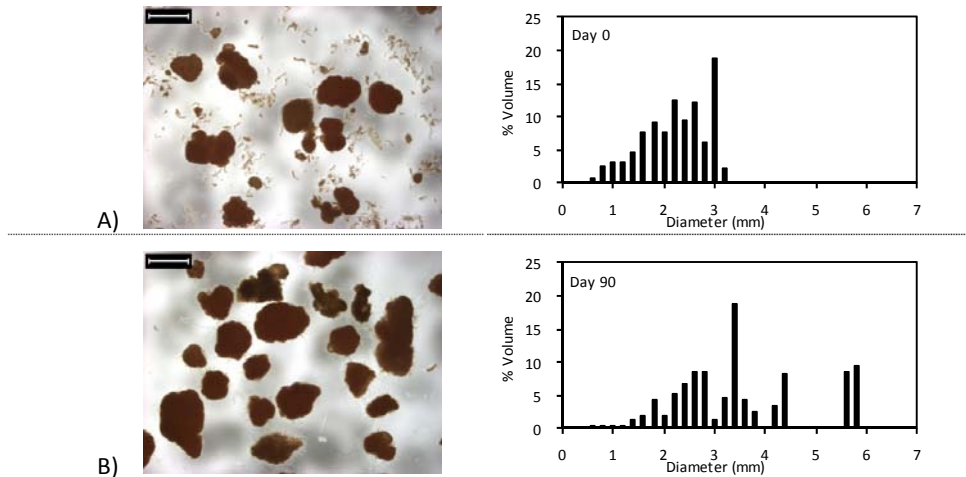
Figure 6.6. Image of the Anammox granules and their volumetric size distribution on days A) 0 and B) 90 of operation.
