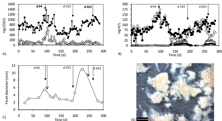
Figure 8.4. Performance of R2 and sampling dates (days 192 and 263) indicated with arrows. A) Organic matter concentration (mg COD/L): COD_{inf} (◆), COD_{eff} (◇); B) nitrogen compounds concentrations (mg N/L): NH_4^+-N_{inf} (●), NH_4^+-N_{eff} (○), NO_2^--N_{eff} (△) in the reactor. C) Evolution of the feret diameter (mm) and breakage episodes indicated with dotted arrows. D) Picture of the granules on day 263 with the bar indicating 2 mm.
