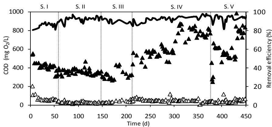
Figure 3.8. Organic carbon concentration in the influent ( \text{COD}_{\text{infr}} , \blacktriangle ), effluent ( \text{COD}_{\text{effr}} , \triangle ) ( \text{mg O}_2/\text{L} ) and removal efficiency percentages ( \text{—} ) (%).
