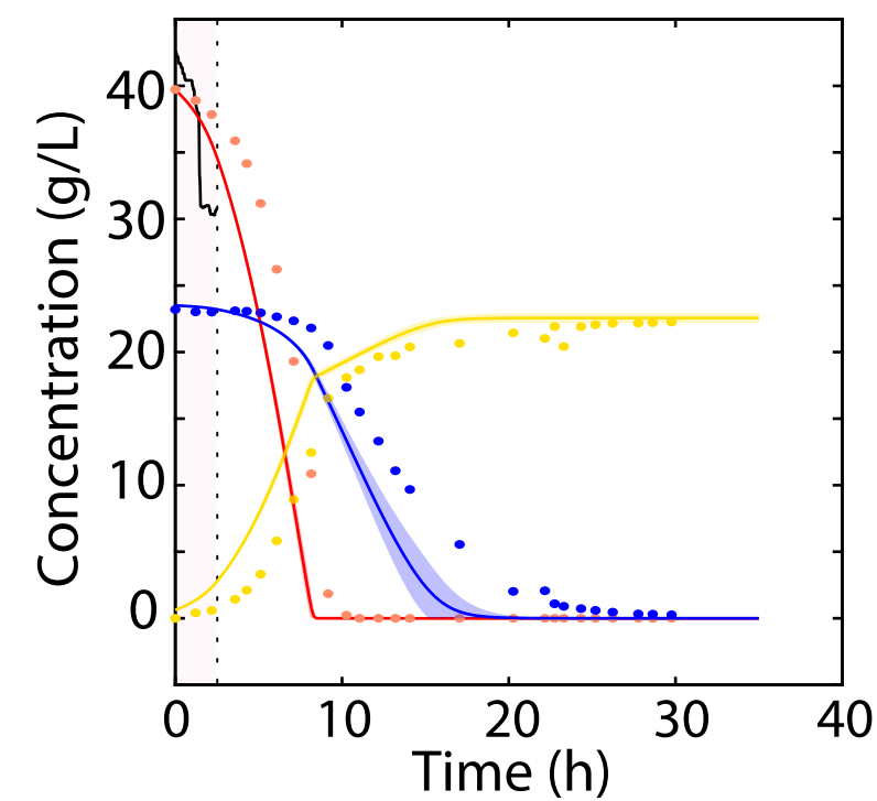
C.3. FERMENTATION 3 (5 h 45 min)
