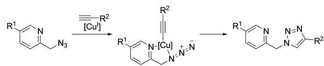
Scheme 3. Pyridine directed CuAAC.
