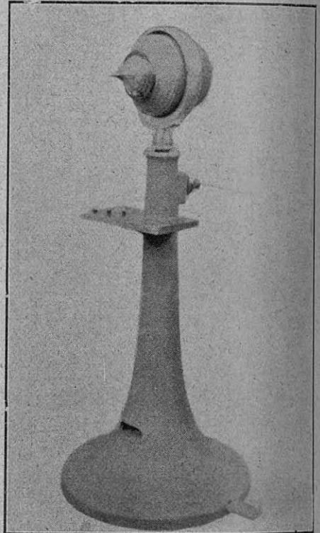
Vista general del electro-imán Haab
