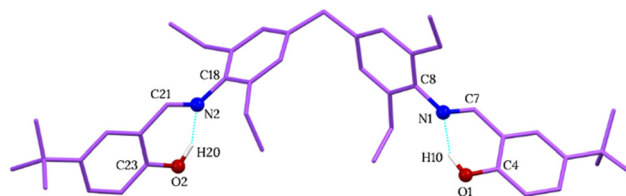
Fig. 2 Stick representation of the ligand \text{H}_2\text{L}^4 4* showing the syn configuration of its branches and the intramolecular hydrogen bonds.
