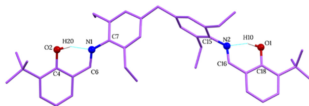
Fig. 3 Stick representation of the ligand \text{H}_2\text{L}^5 5* showing the syn configuration of its branches and the intramolecular hydrogen bonds.
