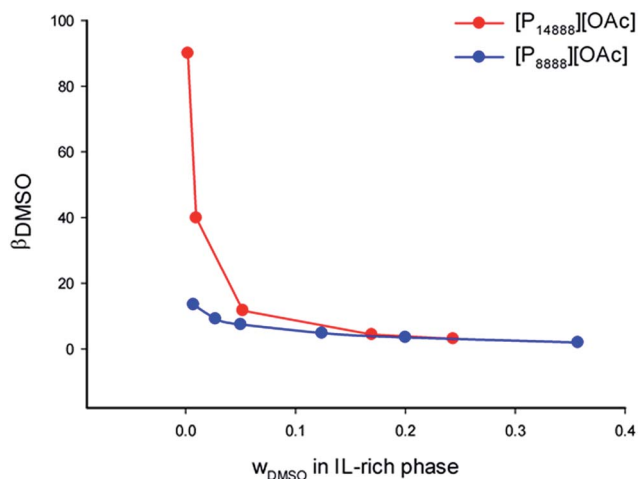
Fig. 6 DMSO distribution ratio ( \beta_{\text{DMSO}} ) for the ternary systems [P_{8888}][\text{OAc}] + \text{DMSO} + \text{water} (blue) and [P_{14888}][\text{OAc}] + \text{DMSO} + \text{water} (red), at 25.0 °C and atmospheric pressure, as a function of the mass fraction of DMSO in the ionic liquid-rich phase.
