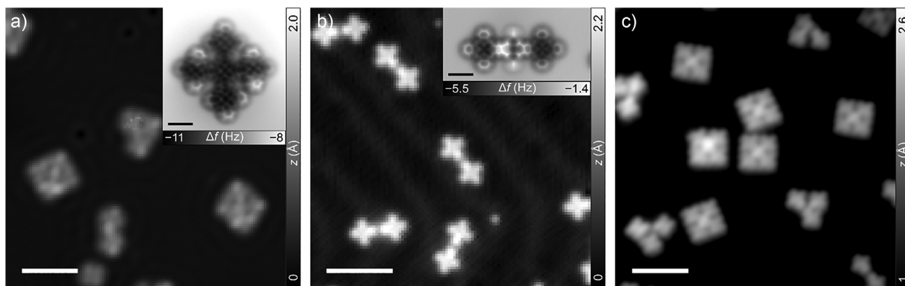
Figure 2. a) Overview STM image of a sample of 2 on Cu(111) after annealing to \sim 520 K for 5 min, showing the successful on-surface synthesis of 1Cu ( V_S = 0.2 V, I = 7 pA). Inset: Bond-resolved AFM image of 1Cu ( V_S = 0 V, \Delta z = -2.15 Å). The AFM image suggests that the overall pentamer structure is non-planar and distorted, which we attribute to its interaction with the substrate. b) Overview STM image of a sample of 2 on Au(111), without co-deposited Fe atoms, after annealing to \sim 570 K for 5 min. Only dimers of 2 can be found on the surface ( V_S = 0.2 V, I = 1 pA). Inset: bond-resolved AFM image of one such dimer ( V_S = 0 V, \Delta z = -1.50 Å). c) Overview STM image of a sample of 2 on Au(111), with co-deposited Fe atoms, after annealing to \sim 520 K for 10 min. Several pentamers 1Fe can be found on the surface. Metal tips were used for STM images. Scale bars in STM images are 5 nm. Scale bars in AFM images (insets) 1 nm.
