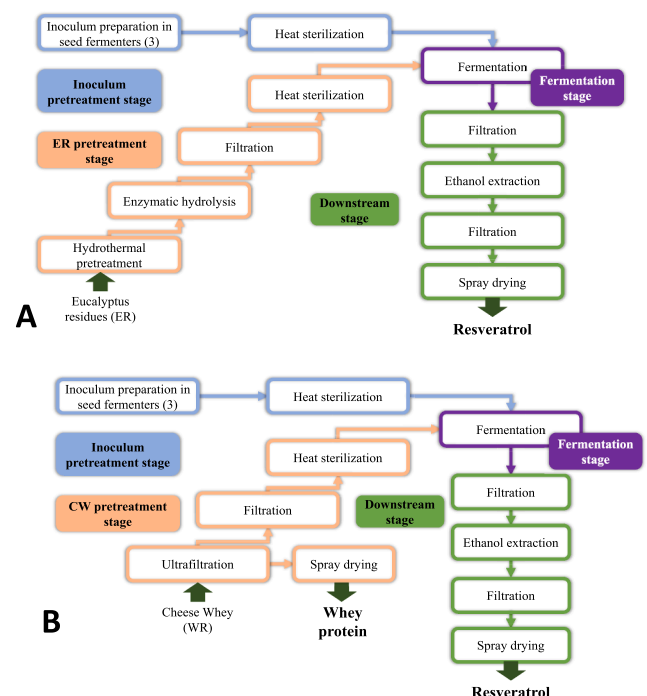
Fig. 1. Resveratrol production pathway (left figure) and process flow diagrams for eucalyptus residues (A) and cheese whey (B) valorization for resveratrol production (right figure).
