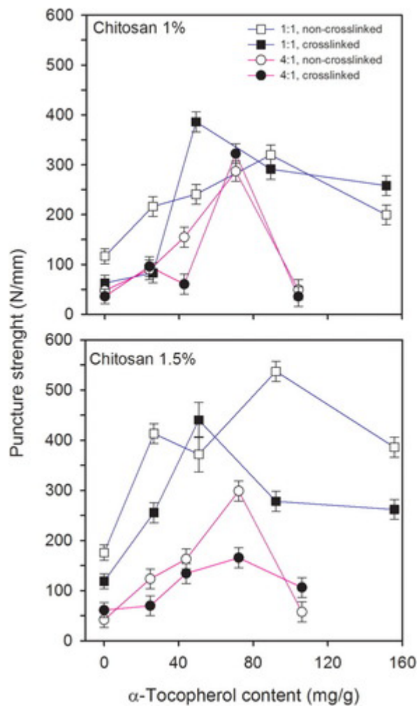
Figure 3. PS estimated as maximum force recorded before the rupture of the films normalized by their thickness according to the ASTM D6241-04 method. The AM : \alpha -tocopherol weight ratio is indicated in the legend. The lines are just a guide for the eye.
