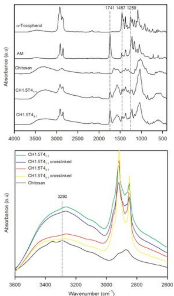
Figure 2. IR spectra of the raw materials and the chitosan films prepared with AM : \alpha -tocopherol 1 : 1 and 4 : 1 weight ratio, before and after cross-linking. Codes as in Table I.
