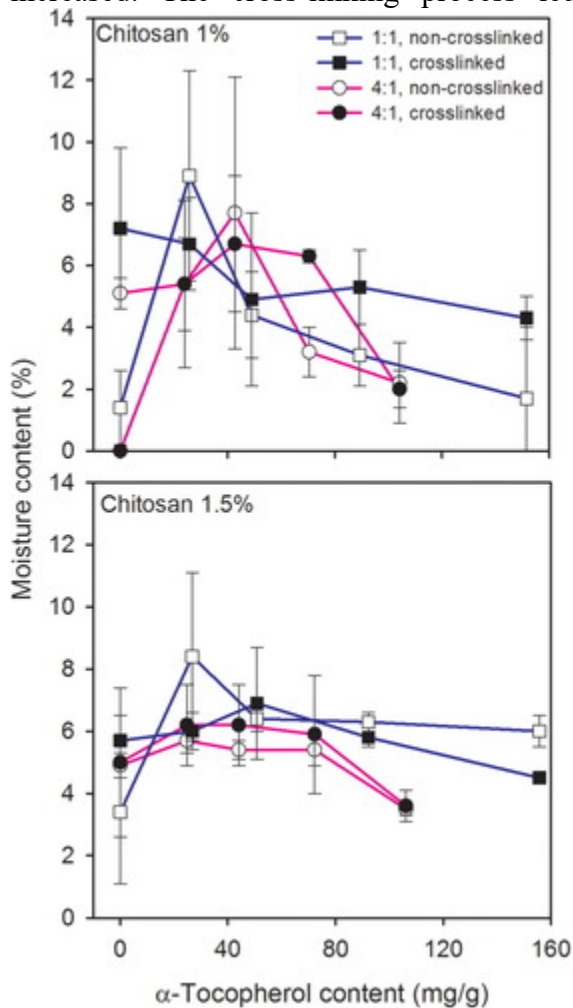
Figure 5. Equilibrium moisture content of films prepared with different AM : \alpha -tocopherol weight ratios and stored at 25°C in an environment of 50% RH.
