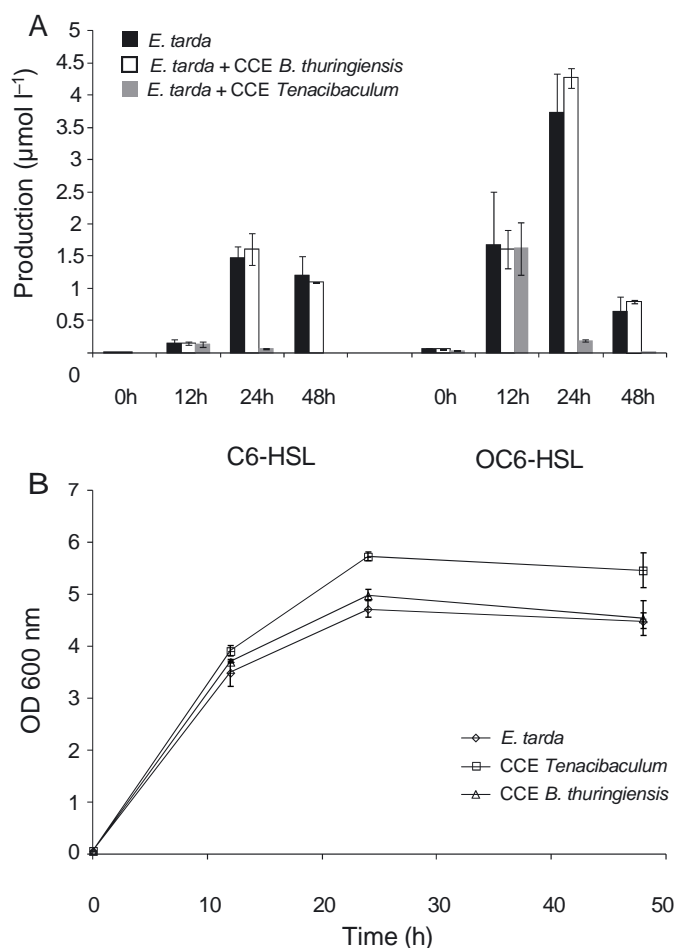
Fig. 4. Edwardsiella tarda ACC35.1. (A) Production of N -hexanoyl-L-homoserine lactone (C6-HSL) and N -oxohexanoyl-L-homoserine lactone (OC6-HSL) by cultures with or without addition of crude cell extracts (CCEs, 100 µg ml -1 ) from Tenacibaculum sp. strain 20J or Bacillus thuringiensis serovar Berliner ATCC10792. (B) Growth curves with or without addition of CCEs. Data are means ± SD of 3 independent cultures
