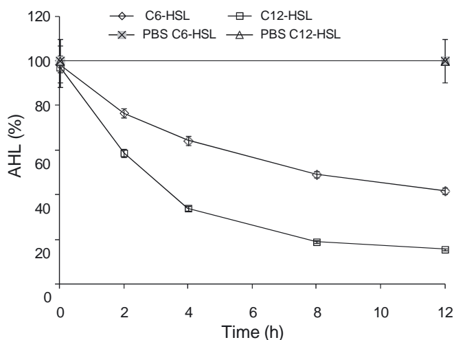
Fig. 3. Tenacibaculum sp. Kinetics of 50 \mu M N -hexanoyl-L-homoserine lactone (C6-HSL) and N -dodecanoyl-L-homoserine lactone (C12-HSL) degradation by crude cell extracts (CCEs) from Tenacibaculum sp. strain 20J obtained in PBS. Controls were set with the signals in PBS. Data are means \pm SD of 3 independent degradation reactions
