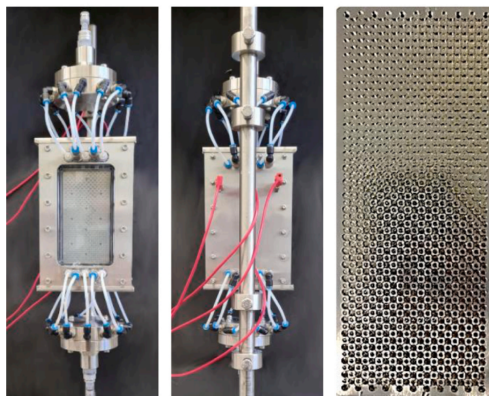
Fig. 1. (a) Sketches of the e^- NETmix reactor disassembled (left) and assembled (right) (frontal views), and (b) pictures of the e^- NETmix reactor assembled (left – frontal view; center – back view) and picture of the electrode plate with the NETmix engraved (right). The e^- NETmix reactor is equipped with a bare fluorine-doped tin oxide (FTO) glass anode.
