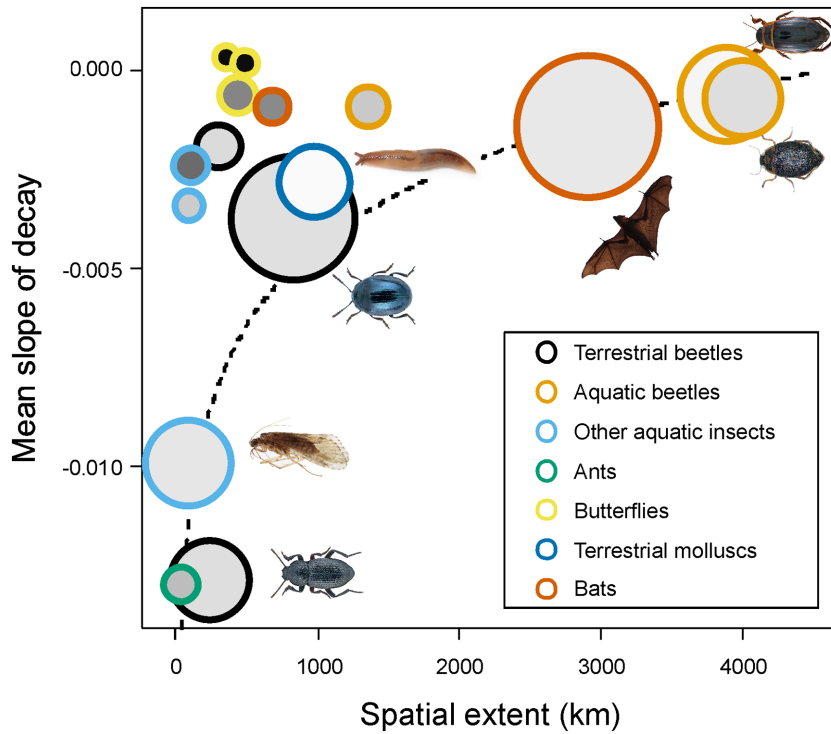
Figure 5. Relationship between distance–decay slope (mean value across genealogical scales) of the distance–decay pattern and spatial extent (maximum distance between sites in each empirical dataset). Summary statistics are indicated by the circle filling shade ( cv_b , variability of slopes across genealogical scales, from low variability = light grey to high variability = dark grey) and circle size ( mean.r^2 , fit of decay curves across scales), showing that datasets presenting a genealogical invariance of distance–decay patterns occupy a specific region in the space defined by dispersal rate (slope of decay) and geographical extent. The dashed line is the logarithmic relationship ( r^2=0.79 , F_{1,5}=19.36 , p=0.007 ) between slope and extent for those datasets in which genealogical invariance was observed (marked with pictures).
