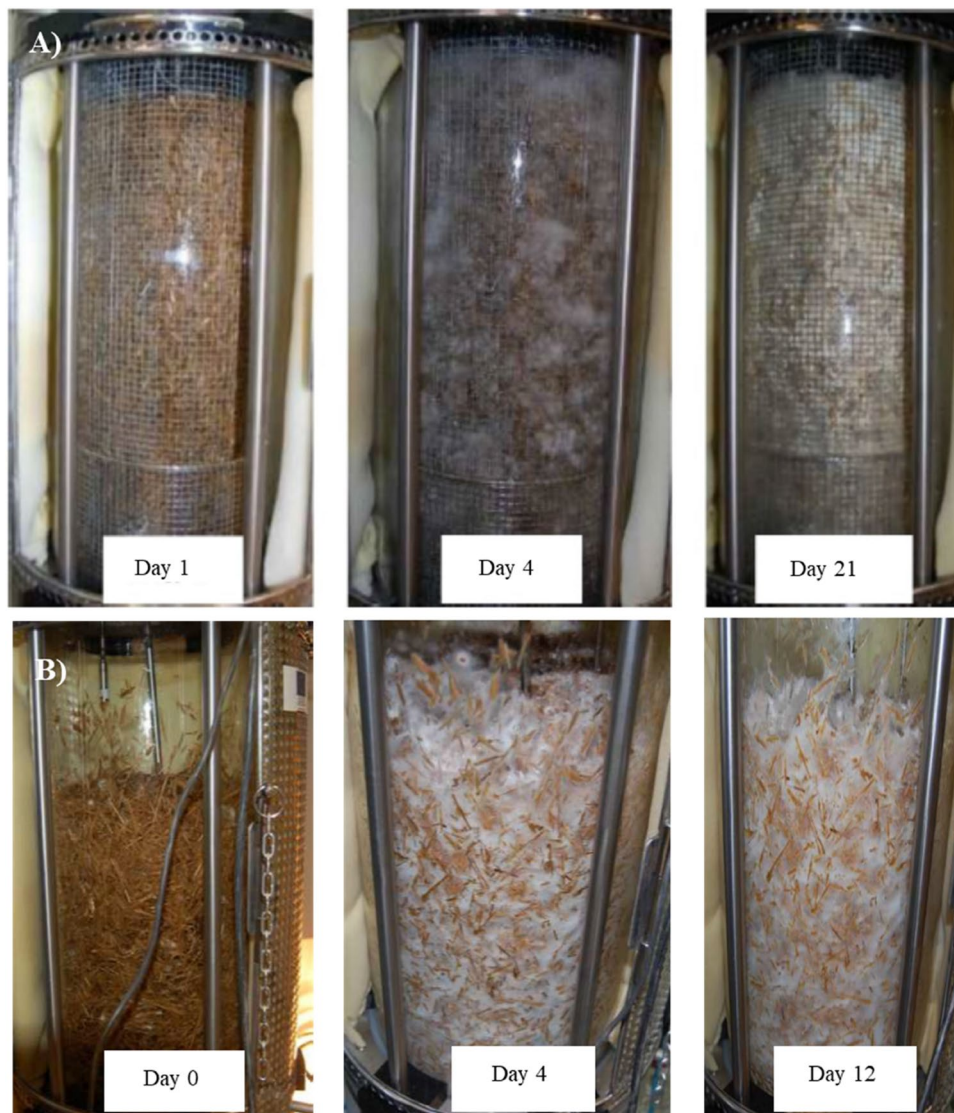
Fig. 2 Evolution of wheat straw during biological pretreatment with I. lacteus in the SSF reactor using the basket (A) and packed bed (B) configurations
