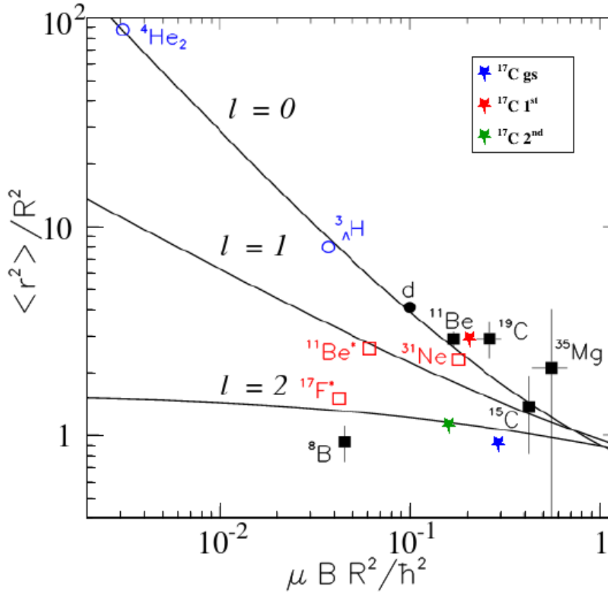
Figure 5.13: Dimensionless radius of the system versus dimensionless binding energy, defined according Riisager's scaling law for two-body halo systems. Black circle represents the deuteron, open blue circles and red squares stand for model estimates and theoretical calculations respectively, while black squares are deduced from experimental data. Blue, red and green stars represent the ground, the first and second excited states in {}^{17}\text{C} (Adapted from [91])
