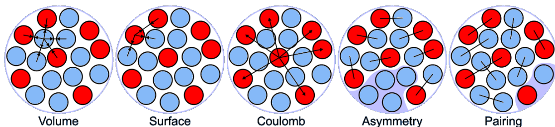
Figure 2.1: Schematics of the 5 terms involved in the semi-empirical mass formula.
