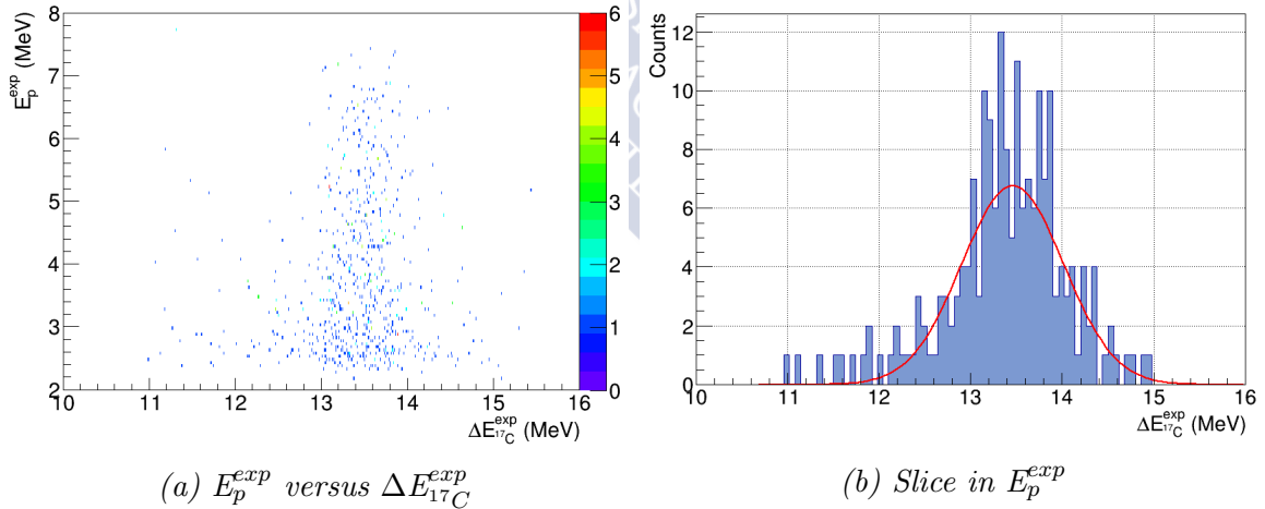
Figure 4.26: Proton energy measured in TIARA, E_p^{exp} , versus ^{17}\text{C}^* energy loss in the first layer of CHARISSA, \Delta E_{^{17}\text{C}}^{exp} (a). In order to obtain a pair of (\Delta E_{^{17}\text{C}}^{exp}, E_p^{exp}) correlated values, a thin slice around E_p^{exp} is projected in the X-axis and fitted with a Gaussian to determine the corresponding \Delta E_{^{17}\text{C}}^{exp} value (b). Due to the lack of statistics, only one point at low energy was taken.
