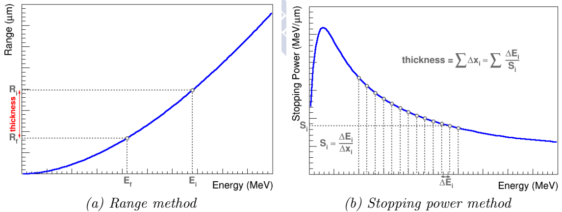
Figure 4.3: Methods of target thickness measurement: the range technique (a) provides the target thickness as the difference between the range at the incident energy and the one corresponding to the residual energy after passing through the target. The stopping power approach (b) consists in dividing the energy loss in small intervals, \Delta E \approx 1 keV, over which the stopping power S is assumed to be constant. Therefore, the total target thickness is then obtained by summing all the small thicknesses of the different energy loss intervals.
