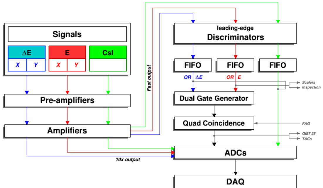
(a) CHARISSA electronic scheme
