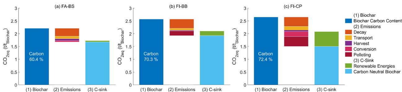
Fig. 2. The bar (1) carbon content, bar (2) related emissions with its production and utilisation, and bar (3) the carbon-sink potential of the produced biochars, from the three different conversion units (a) FA-BS, (b)FI-BB and (c) FI-CP (source: own elaboration).
