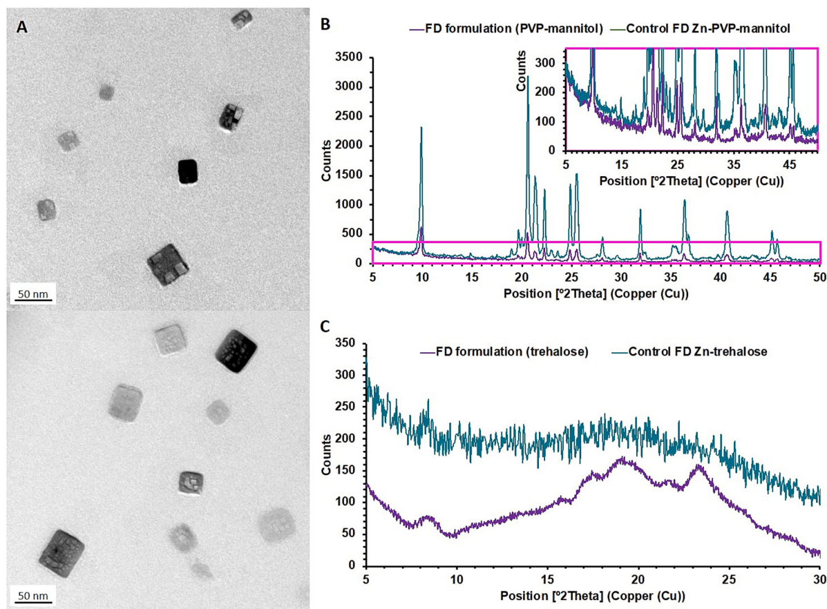
Fig. 2. Characterization of the inner crystalline nanocomplex structure. X-ray analysis was performed to assess whether the nanocomplexes presented the known crystalline structure [30] of the insulin-Zn hexameric complex. A, TEM imaging of nanocomplexes showing inner structural patterns. B, X-ray diffractogram of nanocomplexes freeze-dried with PVP-mannitol (purple line) and control sample of the freeze-dried solution of PVP-mannitol and zinc (green line) at the same concentrations as in the formulations. The diffractogram of the nanocomplexes (purple line) presented several narrow peaks coincident with those of the zinc control sample (green line), which indicated the nonnanocrystalline domains attributed to mannitol. However, the formulation powder also presented wider peaks attributable to nanocrystalline domains, which were not present in the zinc control sample diffractogram, where higher narrower peaks appeared instead (14 to 18°2Th and 23 to 24°2Th). C, X-ray diffractogram of nanocomplexes freeze-dried with trehalose (purple) and control samples of freeze-dried trehalose and zinc (green line). The absence of crystalline phases for the control trehalose-zinc sample (green line) allowed more accurate identification of crystalline domains for the freeze-dried formulation (purple line). The diffractogram of nanocomplexes freeze-dried with trehalose (purple line) presented several wide peaks or bands indicative of nanocrystalline domains, attributed to the nanocomplex core structure. (For interpretation of the references to colour in this figure legend, the reader is referred to the web version of this article.)
