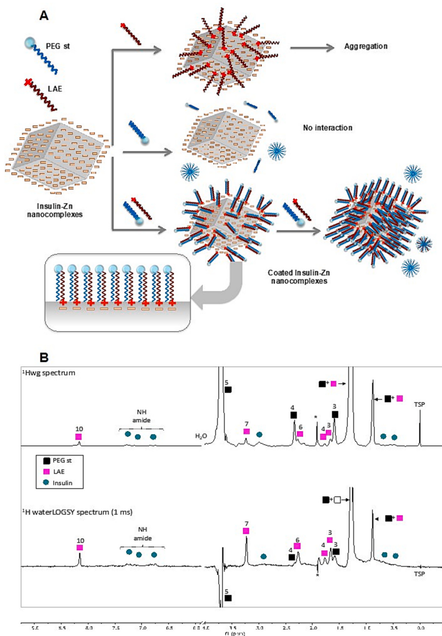
Fig. 3. Characterization of the surfactant bilayer envelope. A, Schematic picture showing the hypothesized conformation of the bilayer of amphiphilic biomaterials based on experimental results. B, ^1\text{H} NMR and waterLOGSY (water-ligand observed via gradient spectroscopy) analysis of the enveloped nanocomplexes. Detailed ^1\text{H} NMR signal assignment and diffusion-ordered spectroscopy (DOSY) experiments disregarding the influence of surfactant molecules not attached to the nanocomplex surface are available in the SI section. The waterLOGSY spectrum clearly showed a 3.71 ppm inverted peak corresponding to PEG regions, while the signal corresponding to bulk aliphatic chains from both surfactants (1.27 ppm) remained noninverted. The observed changes in the signals were proportional to the length of the applied pulse (from 3 to 1 ms, SI section), thus confirming that they were due to the waterLOGSY effect. This observation indicated the external location of the PEG regions and internal location of the aliphatic chains, supporting the hypothesized envelope bilayer architecture.
