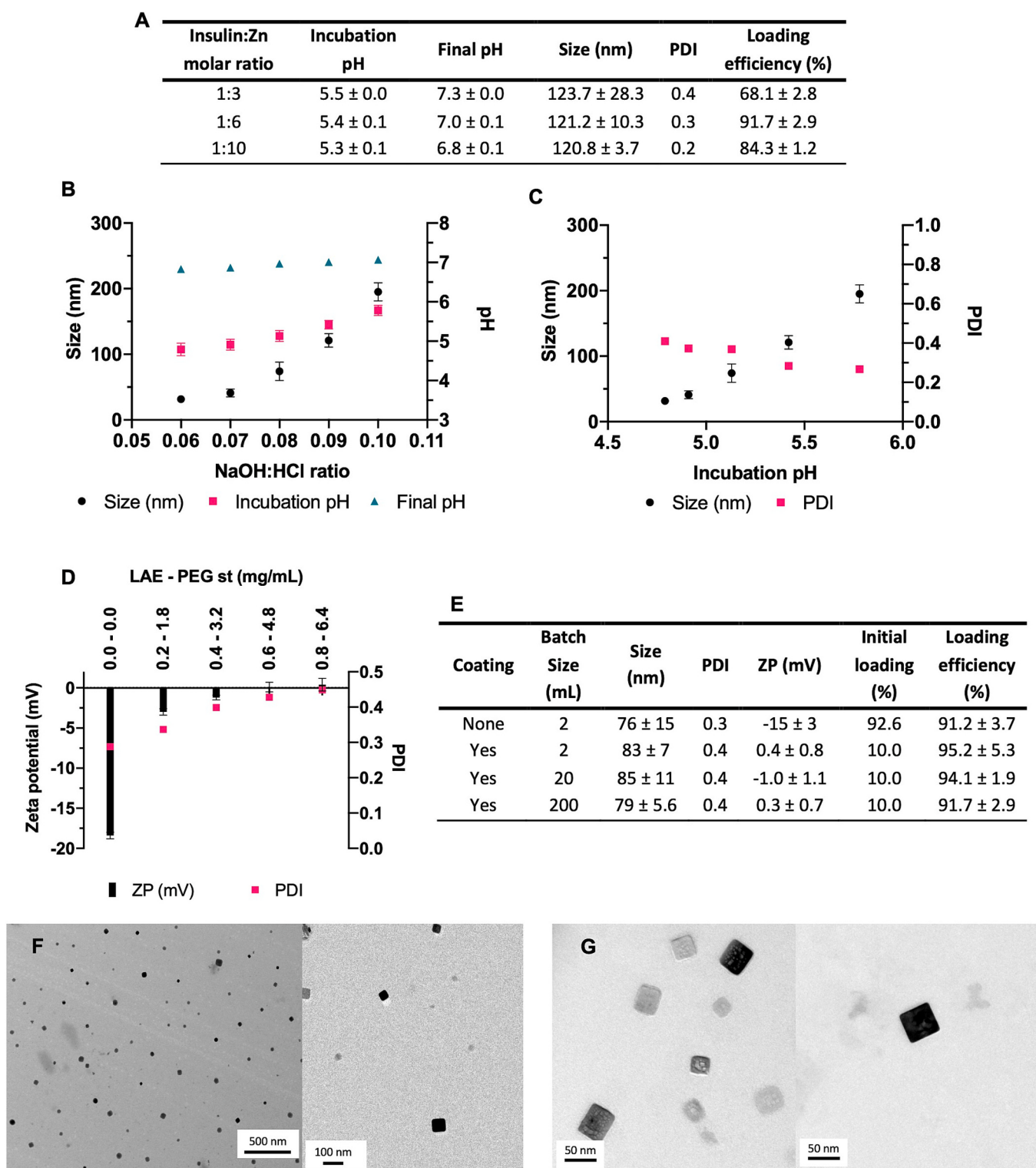
Fig. 1. Bottom-up production of enveloped nanocomplexes. A, pH values adjusted during the production process and resulting physicochemical parameters of the formulations as a function of the employed insulin:Zn ratio. Several ratios [37] were assayed to ensure maximized protein hexameric complexation, and a ratio of 1:6 was finally selected as optimal (over 90 % association). B, pH values in the production process, particle size and PDI measured by DLS of screened formulations as a function of the employed acid-base volume ratios (NaOH 0.1 N: HCl 0.01 N). C, Graphic representation of the particle size and PDI of the formulations as a function of pH at the incubation step. A pH value of 5.1 (NaOH:HCl volume ratio 0.08) was selected for further development, since it allowed us to maintain a small particle size (<100 nm) along with an acceptable PDI value (0.3). D, ZP and PDI values of the nanocomplexes upon addition of increasing concentrations of LAE-PEGst coating, leading to neutral ZP values and increased PDI. E, Physicochemical parameters of formulations before and after coating and upon increasing batch size (10- and 100-fold) after adapting the production process, validating the scaling-up trial. F, TEM images of plain nanocomplexes. G, TEM images of enveloped nanocomplexes. All measurements and error bars are displayed as the mean values ± SDs ( n = 3 ).
