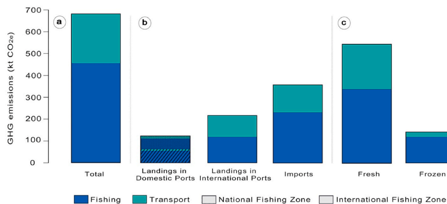
Fig. 4. Total Greenhouse gas emissions (GHG) (kt CO 2 e) for: a) the hake supply chain with breakdown of emissions between fishing and transport to retail, b) by origin of hake considering the catches landed by Spanish vessels in Spanish ports, the catches landed by Spanish vessels in international ports and imports, as well as transportation associated with these categories (the catches landed by Spanish vessels in Spanish ports are divided into catches made in “National fishing zones” and in “International fishing zones”), c) by presentation of hake (fresh and frozen) with breakdown of emissions between fishing and transport to retail.
