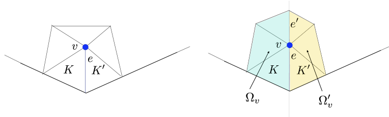
FIGURE 2. Left: sketch of the configuration B(i). Right: sketch of the configuration B(ii). Each time the element K is chosen adjacent to the boundary \Gamma .
