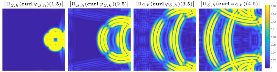
FIGURE 14. Snapshots of the reconstructed S-waves (third experiment).
