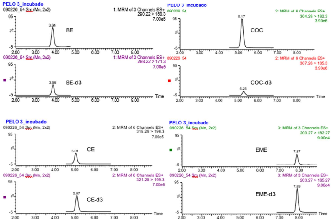
Figure 2. Chromatograms of quantifier MRM transition from sample 3. The concentrations determined were: COC, 2.23 ng/mg; BE, 0.66 ng/mg; EME, 0.036 ng/mg; and CE, 0.17 ng/mg
