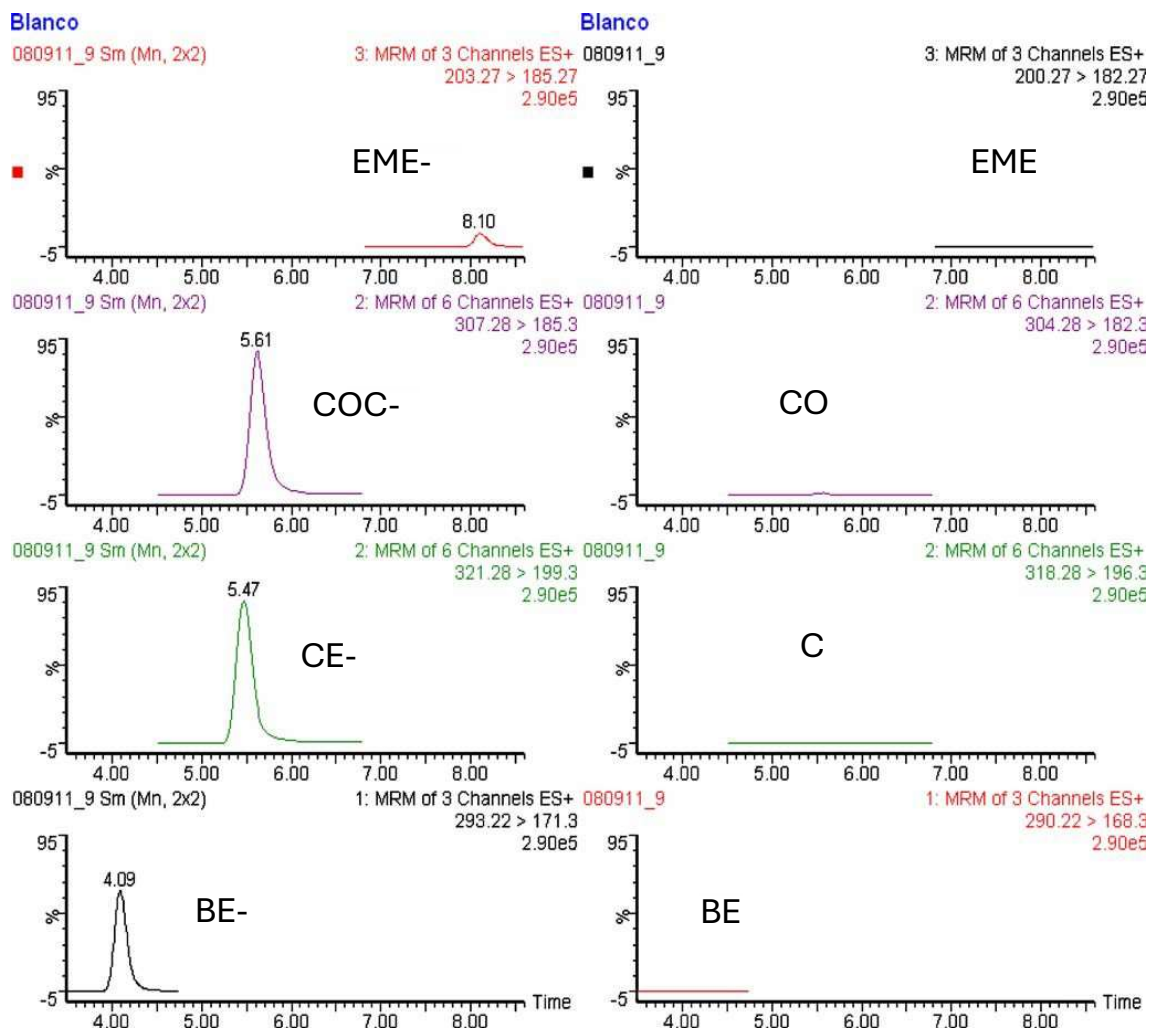
Figure 1. Chromatograms of quantifier MRM transitions of EME, COC, CE and BE and its corresponding deuterated internal standards in a blank hair sample
