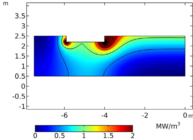
Fig. 6. Power density in the left side of coke bed of a long and thin furnace. The contour lines indicate levels of constant power with a difference of 0.5 MW/m 3 .
