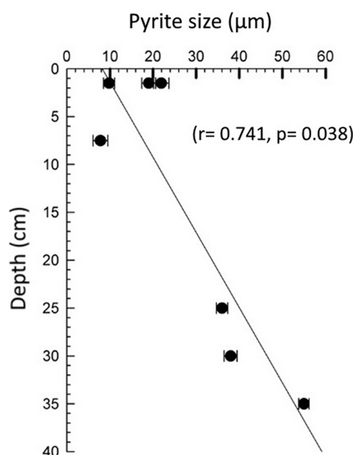
Fig. 8. Correlation between framboidal pyrite size and depth in salt marsh soils.
