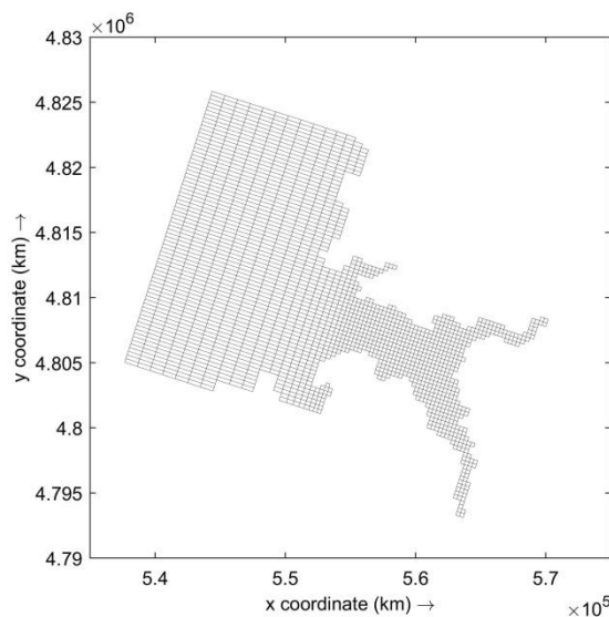
27 28 29 30 31 32 33 34 35 36 37 38 39 40 41 42 43 44 45 46 Fig. 5 - FLOW3D numerical model grid. Only 1 in 3 grid lines are shown for clarity.. Source: own 47 48 49 50 51 52 53 54 55 56 57 58 59 60 61 62 63 64 65
