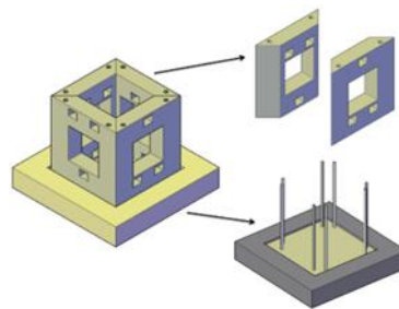
30 Fig. 2- Artificial Reef Module PROARR. Source: Own 31 32 33 34
