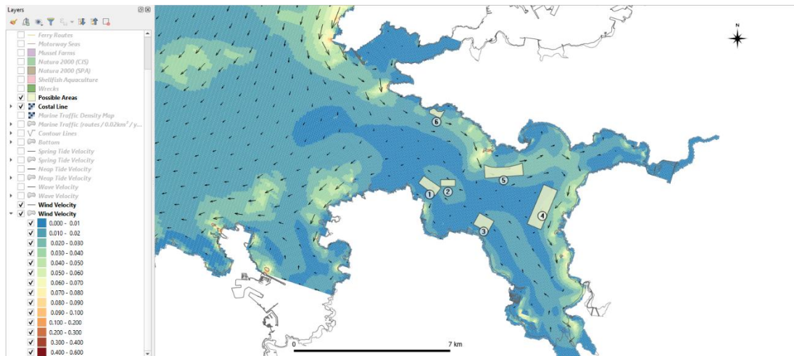
31 Fig. 12- Wind-induced circulation in the Ría de Ares-Betanzos (Case B) (DBMS view). 32 33 34
