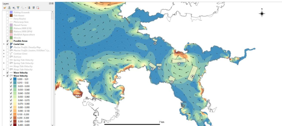
53 Fig. 13- Wave-induced circulation in the Ría de Ares-Betanzos (Case C) (DBMS view). 54
