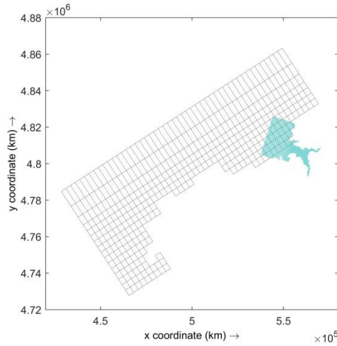
Fig. 6 -SWAN numerical model grids. Only 1 in 3 grid lines are shown for clarity.
