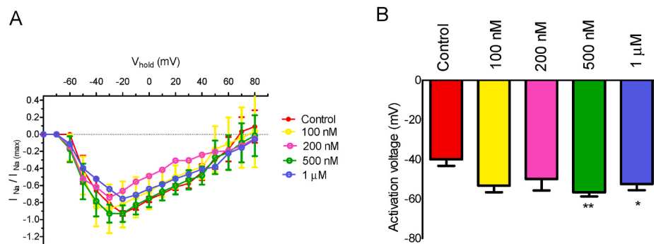
Fig. 6. Effect of MTX3 on sodium currents in HEK Na_v1.6 cells. A. Current-voltage relationship for the effect of different concentrations of MTX3 on sodium currents. B. Voltage activation of sodium currents in absence of toxin, and after application of different MTX3 concentrations.
