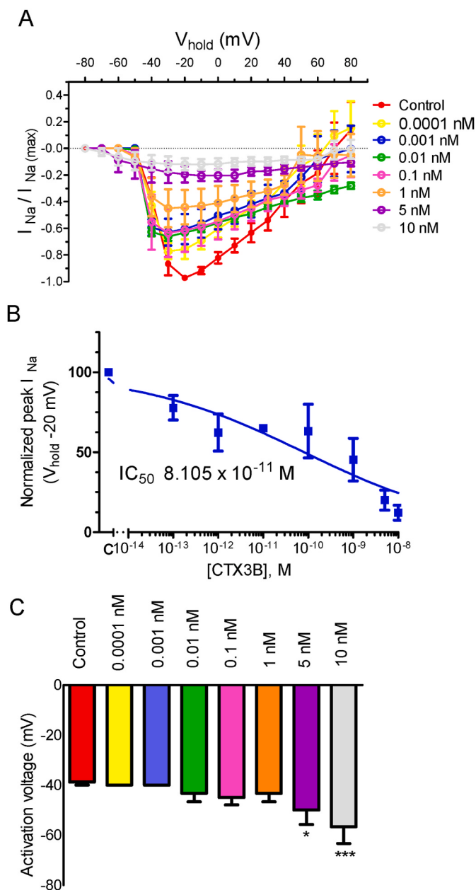
Fig. 4. Effect of CTX3B on sodium currents in HEK Na_v1.6 cells. A. Current-voltage relationship for the effect of different concentrations of CTX3B on the peak amplitude of sodium currents. B. Concentration-response graph indicating the effect of different concentrations of CTX3B on the normalized amplitude of the inward sodium currents. C. Activation voltage of sodium currents in absence of toxin, and after bath application of different CTX3B concentrations.
