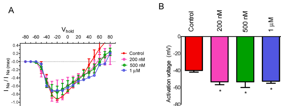
Fig. 7. Effect of gambierone on sodium currents in HEK Na_v1.6 cells. A. Current-voltage relationship for the effect of different concentrations of gambierone on sodium currents. B. Voltage activation of sodium currents in absence of toxin, and after application of different gambierone concentrations.
