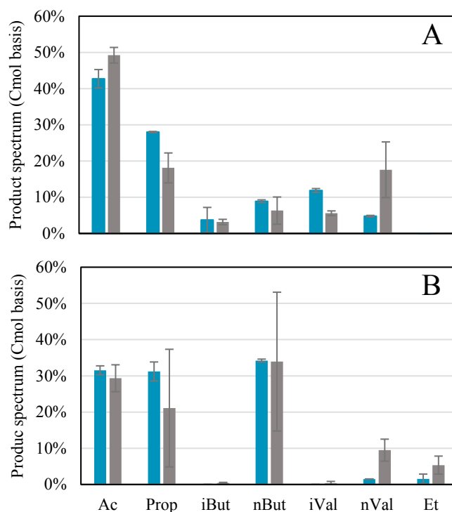
Fig. 4. Product spectra of model and literature results at 3 different D. A: gelatine monofermentation, B: cofermentation. ■ Model results ■ Literature results (Breure et al., 1986).
