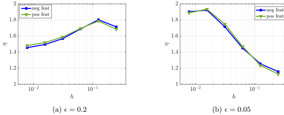
Figure 9: Test 2: effectivity index for the negative and the positive feature cases for two different feature sizes.
