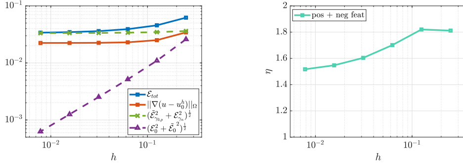
(a) Energy norm of the error and total estimator with its components under mesh refinement. \epsilon = 0.2
