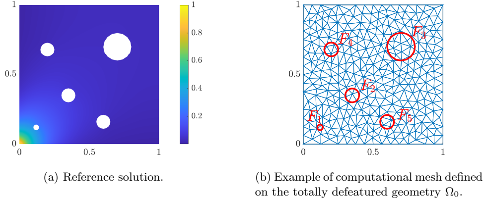
Figure 11: Test 3: reference solution u and totally defeatured geometry \Omega_0 with an example of computational mesh.
