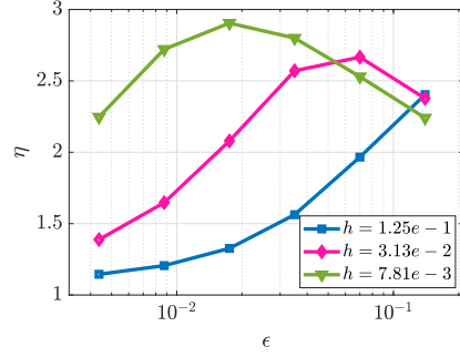
(b) Effectivity index under reduction of feature size, for three fixed mesh sizes.
