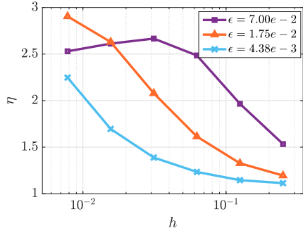
(a) Effectivity index under mesh refinement, for three fixed feature sizes.
