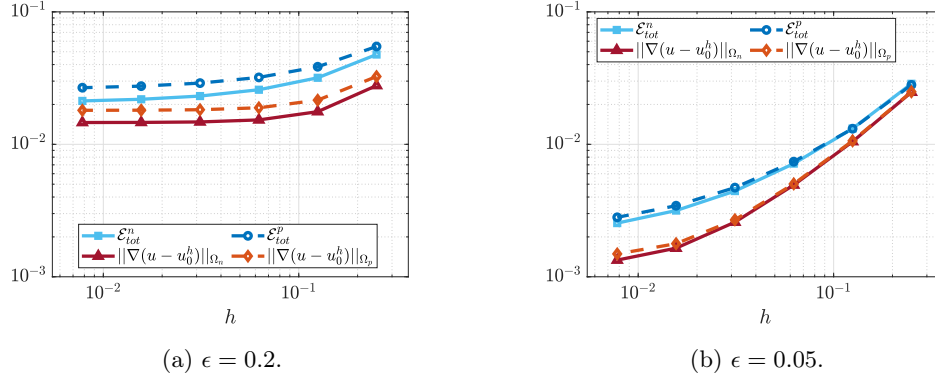
Figure 8: Test 2: energy norm of the error and total estimator under mesh refinement, for the negative and the positive feature cases and for two different feature sizes.
