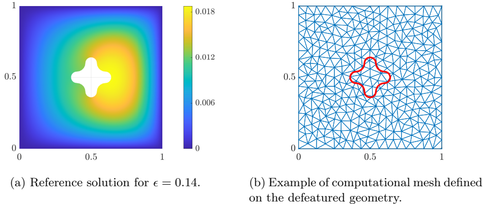
Figure 3: Test 1: reference solution u_\epsilon ( \epsilon = 0.14 ), and defeatured geometry with an example of computational mesh used to compute the defeatured solution and the equilibrated flux reconstruction.
