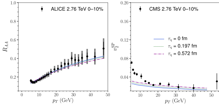
Fig. A.1. (Left) R_{AA}(p_T) , (right) v_2^{\text{SP}}(p_T) for the 0–10% centrality class of \sqrt{s_{\text{NN}}} = 2.76 TeV Pb-Pb collisions at the LHC compared to their respective experimental data [34,57]. The blue solid, \tau_q = 0 fm, dotted green, \tau_q = 0.197 fm, and dashed-dotted purple, \tau_q = 0.572 fm, lines correspond, respectively, to Cases i), ii) and iii) of the early times treatment. DSS07 [48] FFs and T_q = T_{\text{chem}} = 175 MeV are used.
