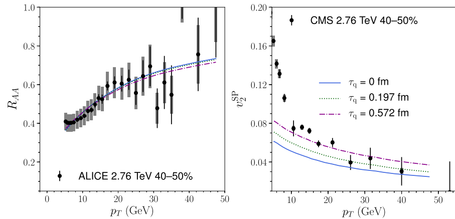
Fig. A.2. (Left) R_{AA}(p_T) , (right) v_2^{\text{SP}}(p_T) for the 40–50% centrality class of \sqrt{s_{\text{NN}}} = 2.76 TeV Pb-Pb collisions at the LHC compared to their respective experimental data [34,57]. The blue solid, \tau_q = 0 fm, dotted green, \tau_q = 0.197 fm, and dashed-dotted purple, \tau_q = 0.572 fm, lines correspond, respectively, to Cases i), ii) and iii) of the early times treatment. DSS07 [48] FFs and T_q = T_{\text{chem}} = 175 MeV are used.
