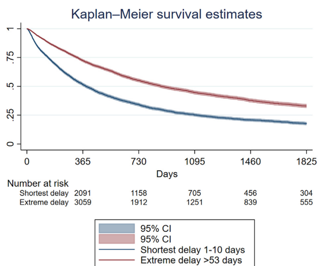
Fig. 1. Kaplan–Meier survival estimates up to five years after diagnosis, comparing survival of cases with the shortest delay and cases with extreme delay.
