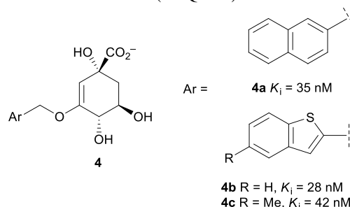
Figure 1. Selected examples of 3-methoxyaryl derivatives that are DHQ2 competitive inhibitors. Inhibition constants against DHQ2-Mt are indicated.
