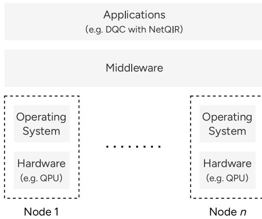
Fig. 2. Levels of a distributed system defined in [35].
