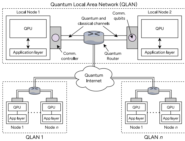
Fig. 4. Complex quantum network architecture interconnecting quantum computing nodes of different QLANs via the Quantum Internet.
