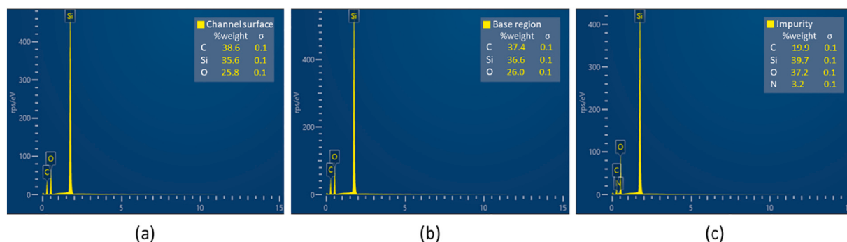
Fig. 11. EDX spectra of the (a) channel surface, (b) base region and (c) impurity observed on the PDMS replica obtained from a Tough resin master.
