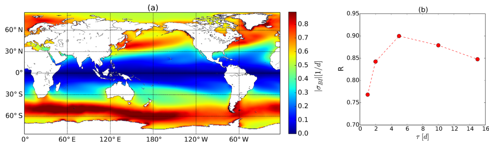
Figure 2. (a) Time average for 35 years of the baroclinic Eady growth rate, Eq. (4), calculated at 850 hPa. (b) Correlation index R between \sigma_{BI} and the 35-year time-averaged forward FTLE map shown in Fig. 1b for different integration times \tau .
