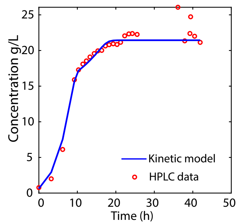
C. ETHANOL
