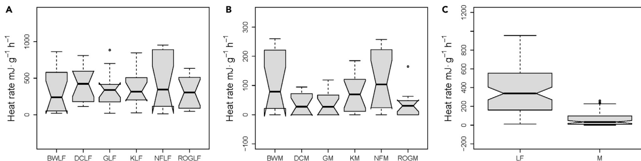
Figure 3. Boxplot notches overlapping for medians of the heat rates
