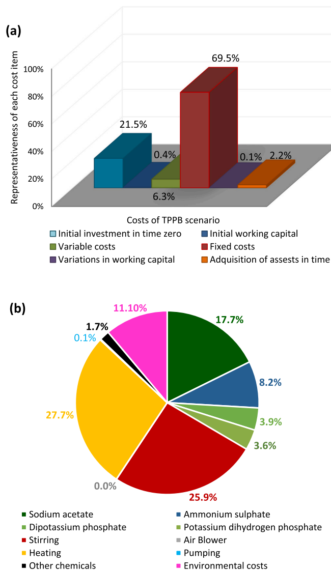
Fig. 6. Economic outcomes of the TPPB scenario. (a) Breakdown per updated cost item; (b) Share of the variable costs of operation.
