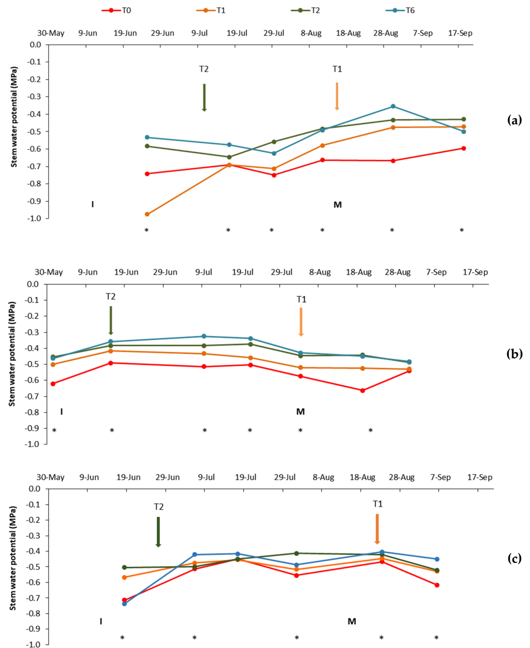
Figure 2. Evolution of stem water potential during the three growing seasons: (a) 2016; (b) 2017; and (c) 2018. Arrows represent the irrigation start date. I, flowering; M, veraison; * indicates significance at p < 0.05 . T0, Rainfed (0% ET 0 ); T1, drip irrigated at 30% ET 0 from the beginning of veraison to harvest; T2, drip irrigated at 30% ET 0 from pea size to harvest; and T6 (control), drip irrigated at 30% ET 0 from budburst to harvest.
