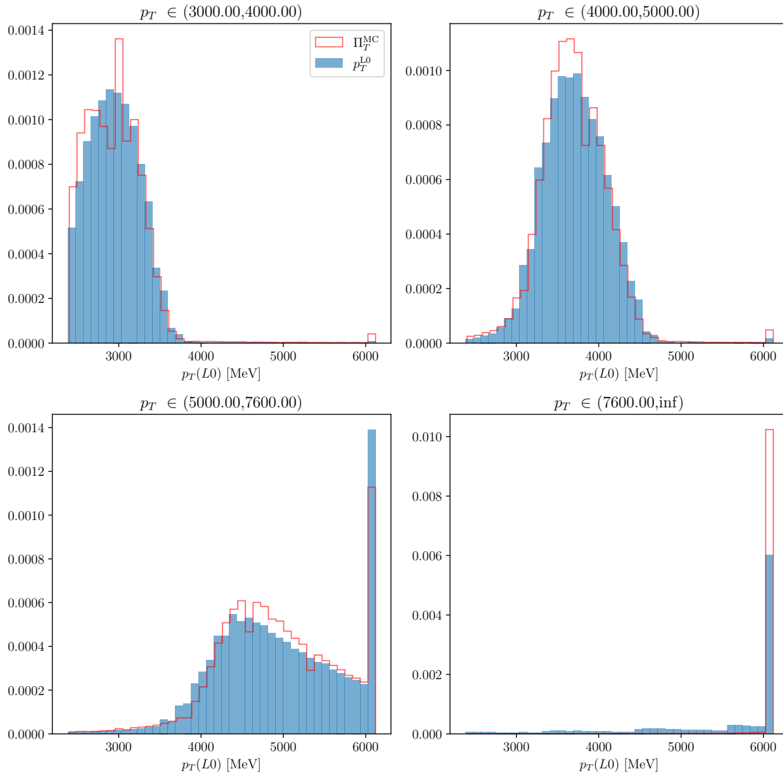
Figure 5.5.7: Comparison between p_T^{\text{L0}} and \Pi_T^{\text{MC}} as closure test using the \eta \rightarrow \mu^+ \mu^- \gamma decay channel in simulation.
