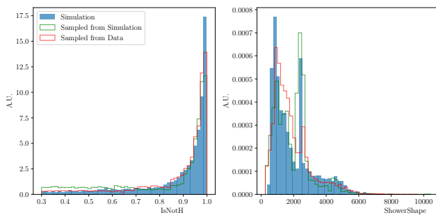
Figure A.2.1: HLT2 IsNotH 5 GeV ALP.
