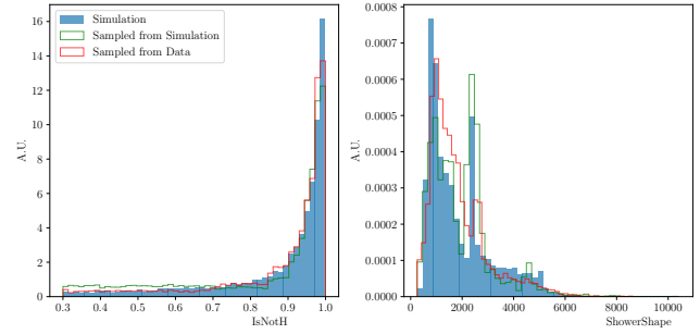
Figure A.2.4: HLT2 IsNotH 8 GeV ALP.
