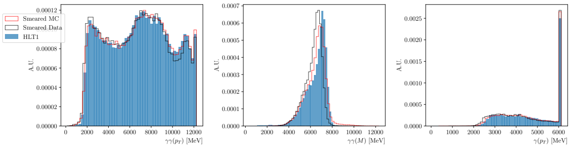
Figure A.1.4: HLT1 kinematic distributions for an 8 GeV ALP.
