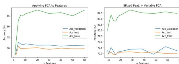
Fig. 1 Average accuracy of the SP classification model across training, validation, and test sets as a function of the number of features ( x -axis), calculated over 100 runs. For scenario (a) (left plot), the features correspond to PCA components derived from the entire feature set. For scenario (c) (right plot), the features consist of 8 fixed features combined with PCA components derived from the remaining features.
