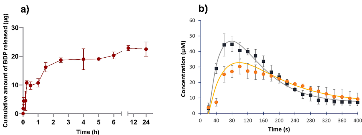
Fig. 6. (a) In vitro release profile ( n = 3 ) of BDP from alginate aerogel carriers in PBS pH 7.4 with 20 % methanol (37 °C, 100 rpm) measured by the classical dialysis method. (b) Drug release profiles ( n = 3 ) of different amounts of BDP-loaded alginate aerogels in the same medium measured by a fast kinetics method. Curved lines correspond to the simulated drug release profiles based on the kinetic model developed by Hirai et.al. and summarized in eq. (3) in Section 2.7 [31]. Symbols: black squares and gray line: experimental and simulated data of 1.5 mg BDP-loaded alginate aerogels, respectively; orange circles and yellow line: experimental and simulated data of 1.0 mg BDP-loaded alginate aerogels, respectively. (For interpretation of the references to color in this figure legend, the reader is referred to the web version of this article.)
