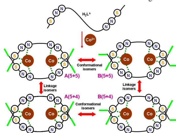
Figure 3. Schematic representation of conformational and linkage isomer mesocates co-crystallised in [\text{Co}_2(\text{L}^a)_2]\cdot\text{CH}_3\text{CN}
