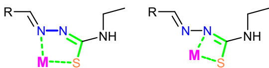
Chart 2. Ambidentate behavior of the hydrazide N-N group in a thiosemicarbazone binding domain
