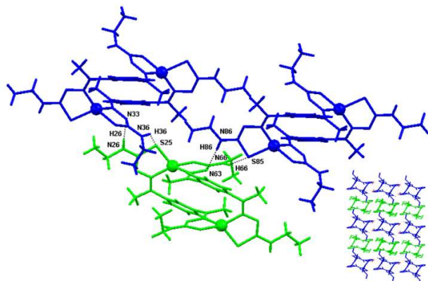
Figure 4. Hydrogen bond interactions between conformational isomers (blue and green) and crystal packing in [\text{Co}_2(\text{L}^a)_2]\cdot\text{CH}_3\text{CN}
