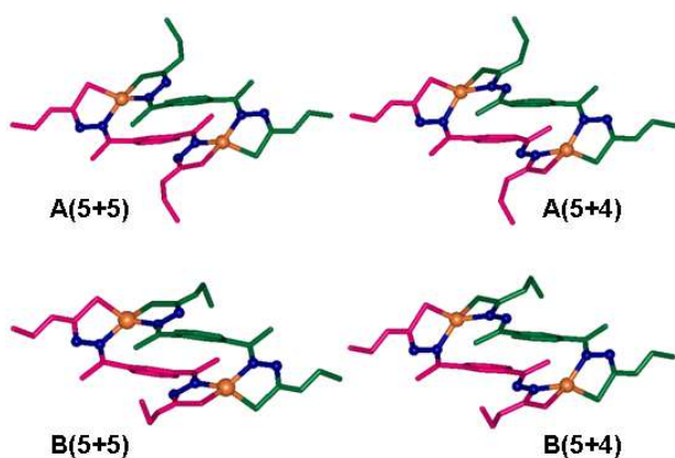
Figure 2. Mixture of conformational [A/B] and linkage isomers [(5+5)/(5+4)] in the crystal cell of the cobalt(II) mesocate [\text{Co}_2(\text{L}^a)_2]\cdot\text{CH}_3\text{CN}
