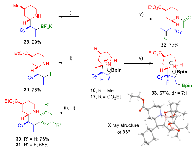
Figure 3. (A–C) Structural modification of products. (i) \text{KHF}_2 (4.5 equiv), \text{MeOH}/\text{H}_2\text{O} 2:1, rt, 3 h. (ii) NIS (1.5 equiv), THF, rt, 2 h. (iii) \text{ArB}(\text{OH})_2 (1.5 equiv), \text{Pd}(\text{PPh}_3)_4 (5 mol %), \text{K}_2\text{CO}_3 (3 equiv), 1,4-dioxane/ \text{H}_2\text{O} 6:1, 100 °C, 2 h. (iv) \text{Cu}(\text{OAc})_2 (1 equiv), \text{Et}_3\text{N} (2 equiv), 4 Å MS, MeCN, 80 °C, 20 h. (v) \text{ICyCuCl} (10 mol %), \text{NaO}^t\text{Bu} (1.2 equiv), \text{B}_2(\text{pin})_2 (1.5 equiv), THF, rt, 16 h. a Ellipsoids shown at 30% probability.
