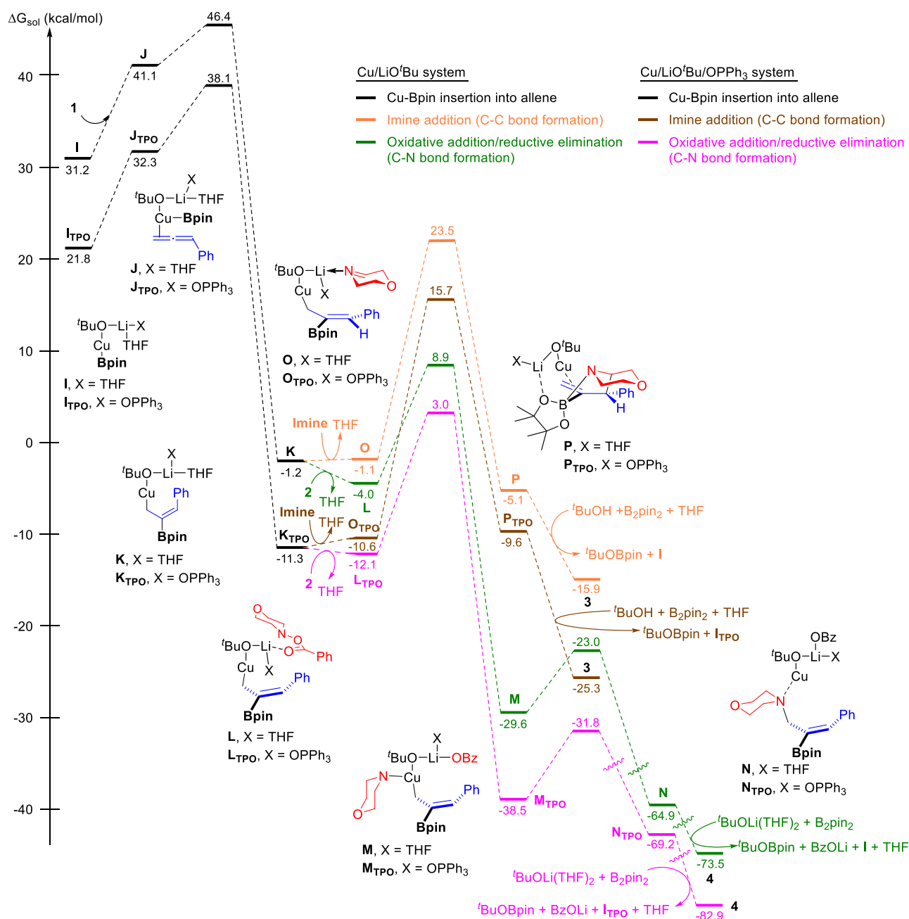
Figure 5. Free energy profile for the pathways leading to the formation of C–C coupling product 3 and C–N coupling product 4 involving dcpe-free copper systems. Computational studies were performed at the B3LYP-D3/6-311++G(d,p)-SDD THF(SMD) //B3LYP-D3/6-31G(d)-SDD level of theory. Energies are relative to complex C combined with those of the relevant substrates.
