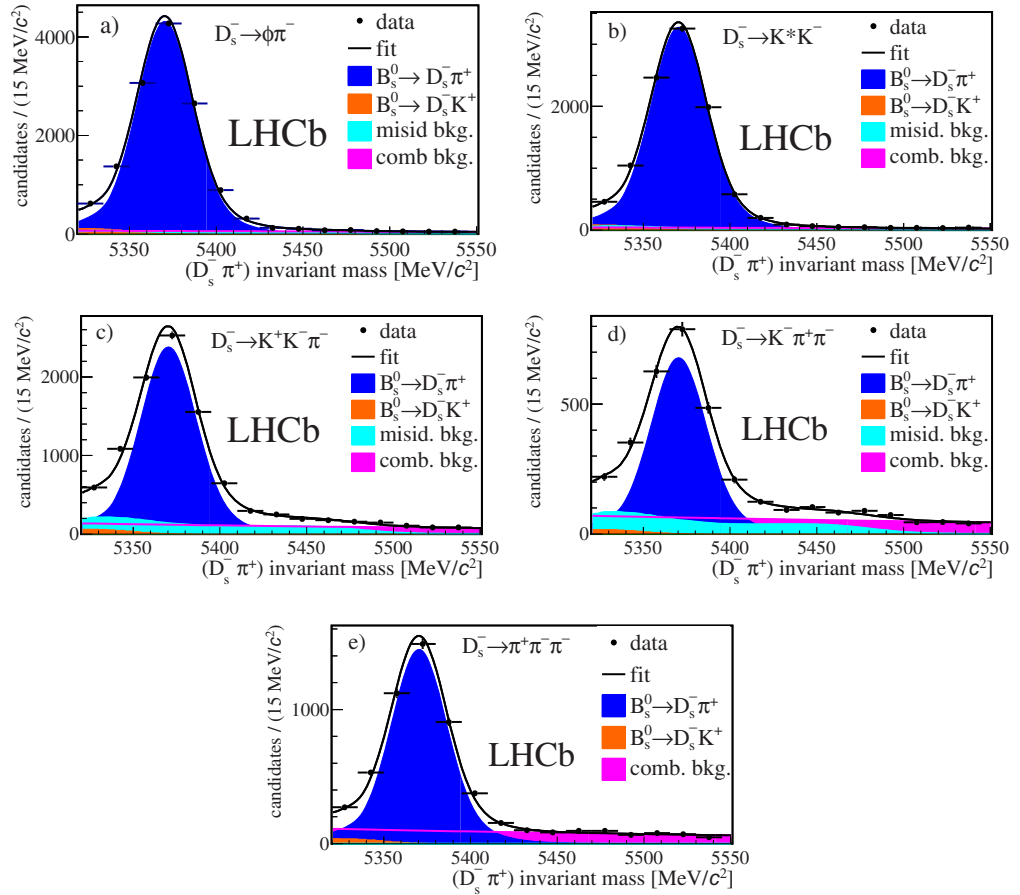
Figure 1. Invariant mass distributions for B_s^0 \rightarrow D_s^- \pi^+ candidates with the D_s^- meson decaying as (a) D_s^- \rightarrow \phi(K^+K^-)\pi^- , (b) D_s^- \rightarrow K^{*0}(K^+\pi^-)K^- , (c) D_s^- \rightarrow K^+K^-\pi^- nonresonant, (d) D_s^- \rightarrow K^-\pi^+\pi^- and (e) D_s^- \rightarrow \pi^-\pi^+\pi^- . The fits and the various background components are described in the text. Misidentified backgrounds refer to background from B^0 and \Lambda_b^0 decays with one misidentified daughter particle.
