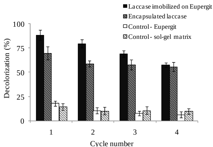
Figure 3.9. Decolorization percentages of AG27 after each consecutive continuous cycle performed in the PBRs with both encapsulated and immobilized laccase on Eupergit supports.
