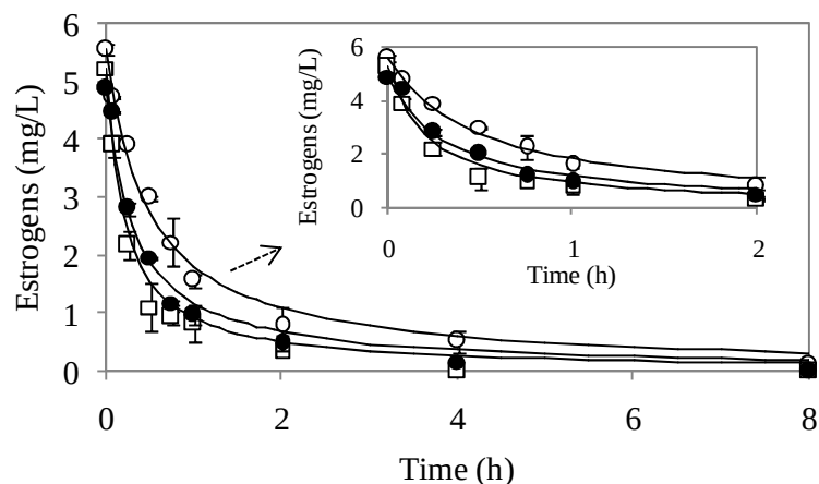
Figure 2.11. Concentrations of E1 (○), E2 (□) and EE2 (●) during the treatment with Myceliophthora thermophila laccase at pH 7. Solid lines represent the fitting of data to second order kinetics.
