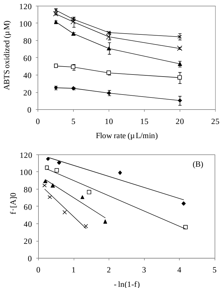
Figure 6.8. (A) Flow rate and concentration effects on the oxidation of ABTS in laccase-immobilized microreactors under continuous flow conditions. Initial concentrations of ABTS tested were: 25 ( \blacklozenge ), 50 ( \square ), 100 ( \blacktriangle ), 250 ( \times ) and 500 \mu\text{M} ( * ). (B) Analysis of the kinetic data collected using Equation (6.1) model. Symbols correspond to: 2.5 ( \blacklozenge ), 5 ( \square ), 10 ( \blacktriangle ) and 20 \mu\text{L}/\text{min} ( \times ) of continuous flow rate. Solid lines fitted by linear regression.
