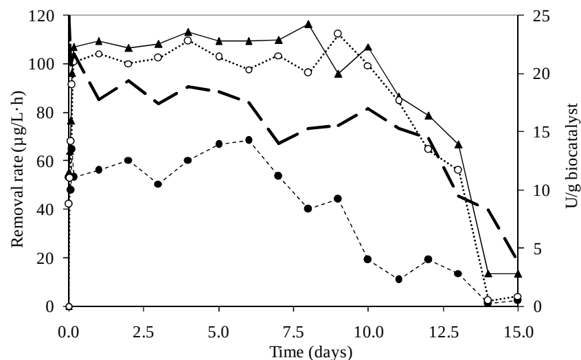
Figure 3.11. E1 (●), E2 (▲) and EE2 (○) removal rates ( \mu\text{g/L}\cdot\text{h} ) attained during the operation of the FBR with immobilized laccase on Eupergit supports, with 100\ \mu\text{g/L} of estrogens and 50 min of HRT. The biocatalyst activity profile during the operation (---) is also shown.
