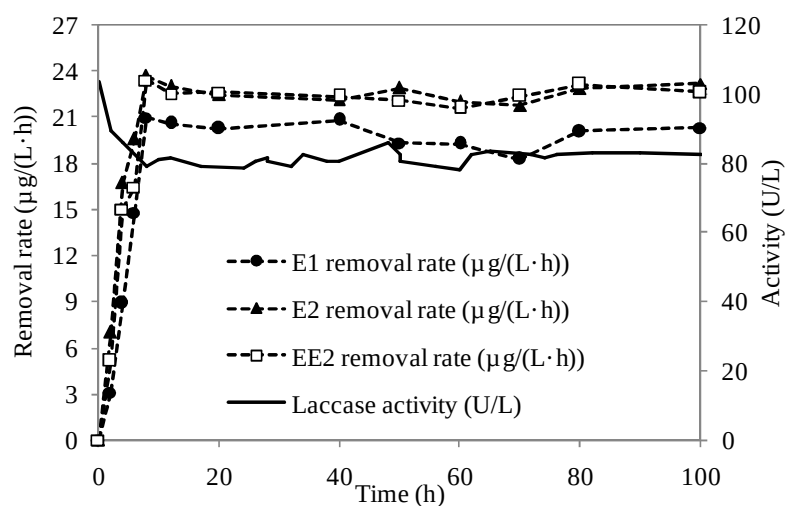
Figure 4.12. E1, E2 and EE2 removal rates and laccase activity during the operation of the 2 L-EMR for the treatment of real wastewater containing 100 \mu\text{g/L} of each estrogen (feed addition rate 25 \mu\text{g}/(\text{L}\cdot\text{h}) ) by 100 U/L of initial laccase activity.
