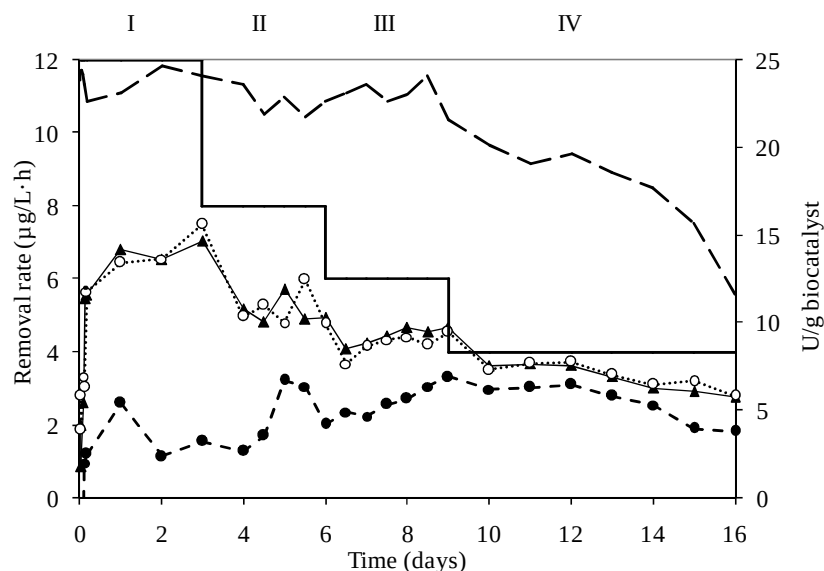
Figure 3.12. E1 (●), E2 (▲) and EE2 (○) removal rates ( \mu\text{g/L}\cdot\text{h} ) attained during the operation of the FBR with immobilized laccase on Eupergit supports, with 10\text{ }\mu\text{g/L} of estrogens and variable HRT between 50 and 150 min (Table 3.1). Feed addition rates (—) and biocatalyst activity (---) profiles are also shown.
