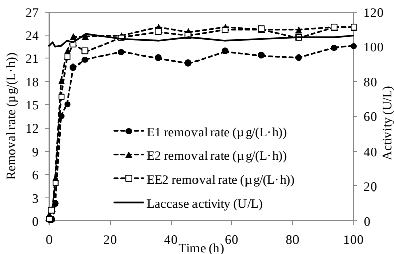
Figure 4.11. E1, E2 and EE2 removal rates and laccase activity during the operation of the 2 L-EMR for the treatment of synthetic waste water containing 100 \mu\text{g/L} of each estrogen (feed addition rate 25 \mu\text{g}/(\text{L}\cdot\text{h}) ) by 100 U/L of initial laccase activity.
