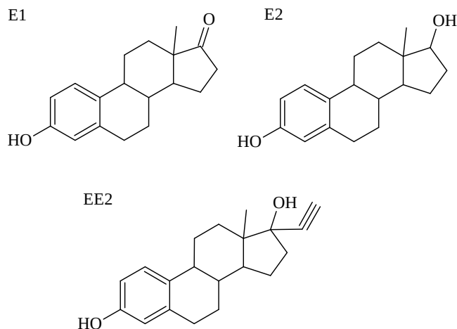
Figure 1.2. Structures of the target estrogenic compounds evaluated in this work.
