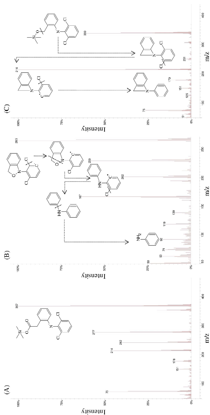
Figure 5.12. Mass spectra corresponding to derivatized and deprotonated DCF (A), deprotonated P1 (B) and derivatized and deprotonated P2 (C) including the proposed fragmentation patterns for the products.
