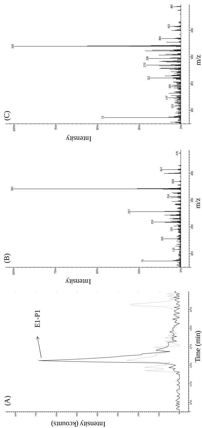
Figure 5.2. Selected ion monitoring chromatogram (m/z 340) for the sample after 8 h of laccase-catalyzed transformation of E1 (black line) and for the corresponding control (grey line) (A) and mass spectra corresponding to E1 (B) and E1-P1 (C) obtained by GC-MS.
