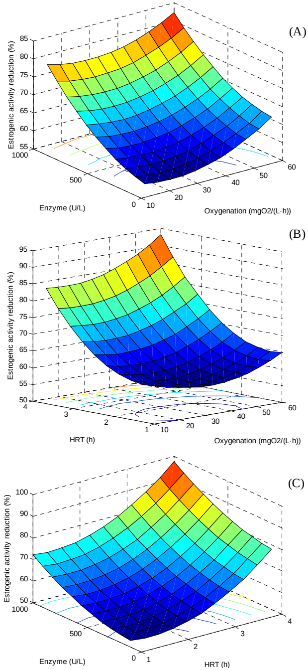
Figure 4.9. Response surface plots for estrogenic activity reduction ( Y_3 , %) as a function of: (A) oxygenation and enzyme activity at HRT 2 h; (B) oxygenation and HRT at 500 U/L; (C) enzyme activity and HRT at oxygenation rate of 30 mg O 2 /(L·h).
