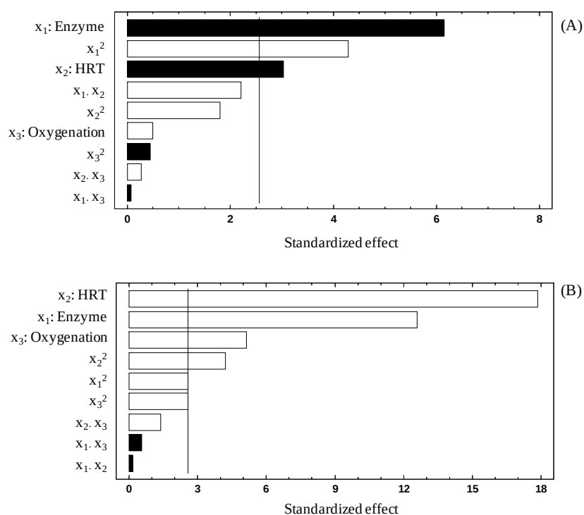
Figure 4.8. Pareto charts for E1 removal rate per units of enzyme used ( Y_2 , mg/(L·h·U)) (A) and for estrogenic activity reduction ( Y_3 , %) (B). Black bars: antagonistic effect; White bars: synergistic effect.
