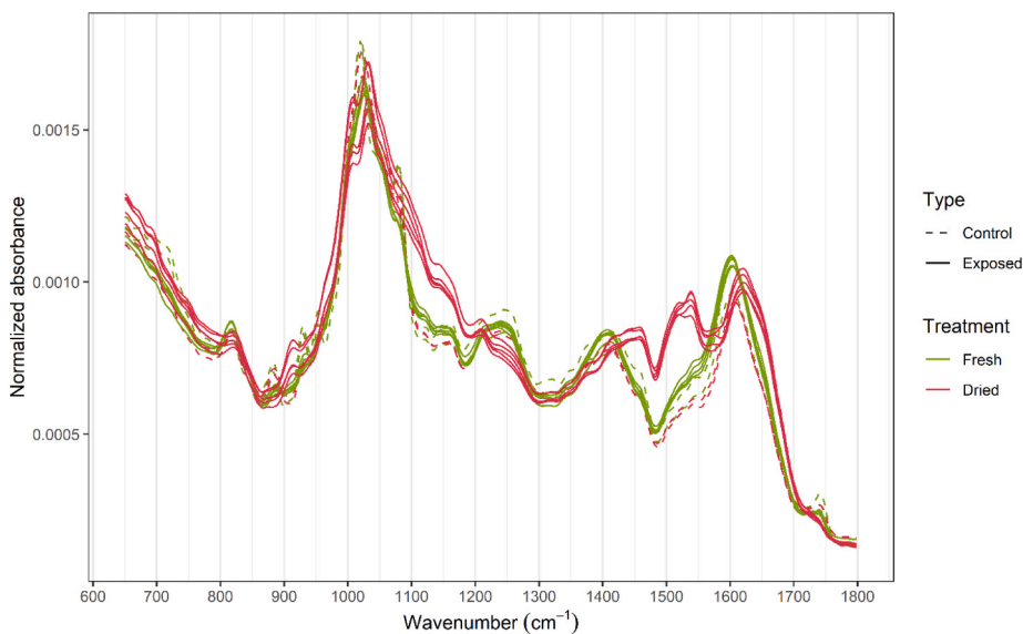
Fig. 3. Normalized absorption spectra of 14 samples in the region from 600 to 1800 \text{cm}^{-1} .
