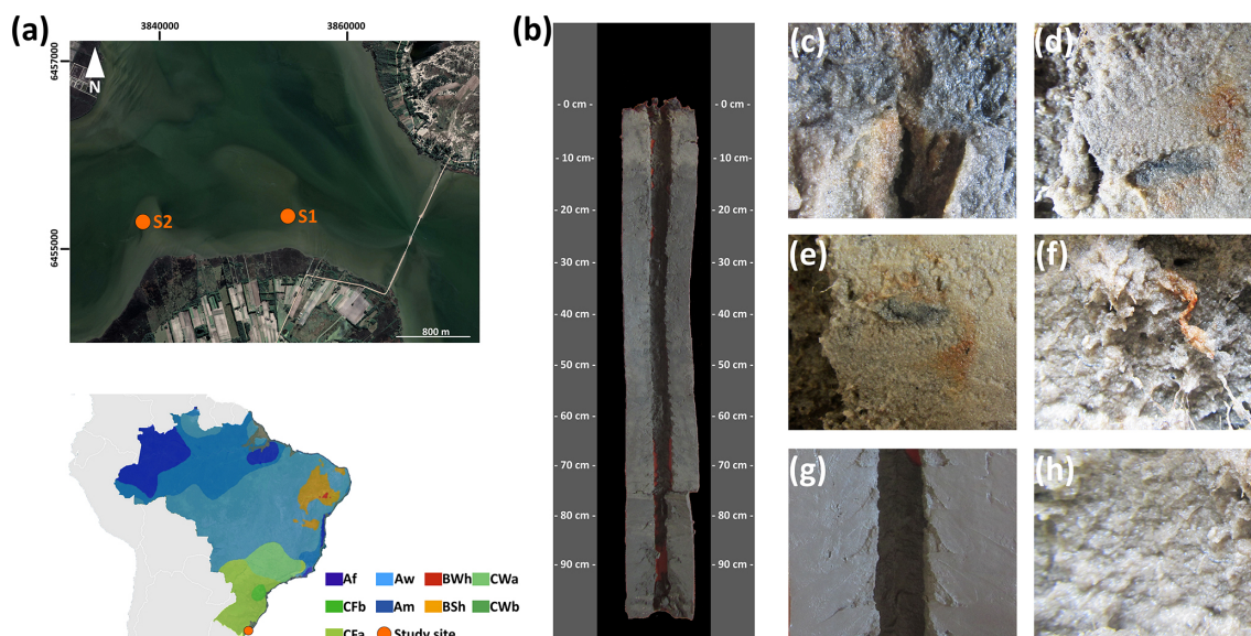
Figure 3. (a) Sampling site location on the southern Brazilian coast and the Köppen–Geiger climatic classification of the studied sites (source: Peel et al., 2007). (b) The representative soil profile of the southern coast (S1, soil horizons Ar 0–6 cm, ACrj 6–13 cm, CAr1 13–30 cm, CAr2 30–44 cm, Cr 44–70 cm, 2Crn1 70–93 cm, 2Crn1/2Crn2 93–106 cm, 2Crn2 106–111 cm) classified as a Eutric Fluvisol Subaquatic Gleysol (Loamic, Protosalic, Sodic, Hypersulfidic). Detailed images of (c) and (d) black-colored spots (10BG 3/1 very dark greenish gray) due to metal sulfides in the Crn2/2Crn, (e) and (f) brown mottles (7.5YR 4/4) associated with roots (oxyhydroxide precipitations), and (g) and (h) contrasting soil textures between horizons 2Crn2 (clay texture) and Ar (loamy fine sand), respectively.
