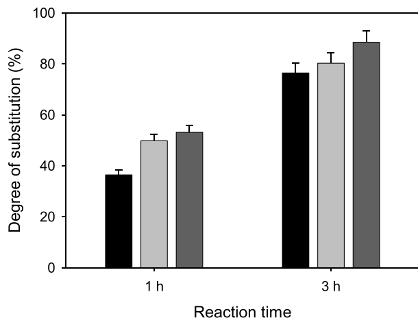
Figure 6. DS in the carboxymethylation of untreated Avicel (black columns) and of Avicel samples pretreated with pure [P_{4444}][OAc] (light gray columns) or with a mixture of [P_{4444}][OAc] + DMSO with x_{DMSO} = 0.20 (dark gray columns) after reaction times of 1 and 3 h. The ATR-FTIR spectra used for the calculation of these DS values are shown in Figure S15 in the Supporting Information.
