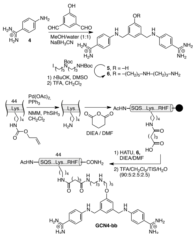
Scheme 2. Top: Synthesis of the bisbenzamide aromatic derivative 6 by reductive amination of 5-hydroxyisophthalaldehyde, introduction of the aminoalkyl side chain in the phenolic oxygen, and acidic deprotection. Bottom: Key steps in the synthesis of GAGA-bb . The black circle represents the solid resin used in the peptide synthesis.
