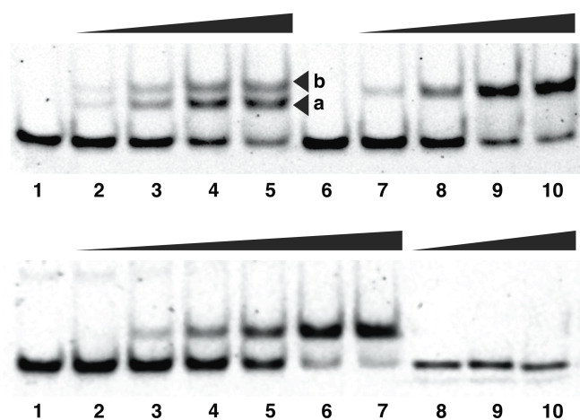
Figure 3. Top: EMSA assays of DNA recognition by GCN4-bb . Lanes 1-5: target API hs •AT dsDNA (50 nM). Lanes 2-5: 100, 300, 500, 800 nM GCN4-bb ; lanes 6-10: control API m •AT dsDNA (50 nM). Lanes 7-10: 100, 300, 500, 800 nM GCN4-bb . Bottom: EMSA assays of DNA recognition by GAGA-bb . Lanes 1-7: target dsDNA AT•GAG (50 nM). Lanes 2-7: 100, 200, 300, 400, 500, 600 nM GAGA-bb . Lanes 8-10: control AT m •GAG dsDNA (50 nM); lanes 9-10: 300, 500 nM GAGA-bb . dsDNA sequences (binding site in italics): API hs •AT : 5'-CGAACG TCAT AAATTT CCTC-3'; API m •AT : 5'-CGAACG TGCT AAATTT CCTC-3'; AT•GAG : 5'-GACGG AATTT GAGAG CGTCG-3'; AT m •GAG : 5'-GACC GGGCC GAGAG TACGT-3'. EMSA assays of DNA recognition by GCN4-bb were done in the same conditions as for GCN4-pr ; in the case of GAGA-bb the buffer used was slightly different (see the supporting information for details).
