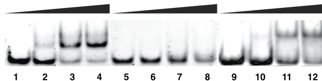
Figure 1. EMSA GCN4-pr DNA binding assays in Tris-HCl buffer. Lanes 1-4; target API bs •AT dsDNA (50 nM), lanes 2-4: 100, 300, 500 nM GCN4-pr ; lanes 5-8: control API bs •GC dsDNA (50 nM), lanes 6-8: 100, 300, 500 nM GCN4-pr ; lanes 9-12: control GC•AT DNA (50 nM), lanes 10-12: 100, 300, 500 nM GCN4-pr . dsDNA sequences (binding site in italics, only one strand is shown): API bs •AT : 5'-CGAACG TCAT AAATTT CCTC-3'; API bs •GC : 5'-ACGAACG TCAT GGCC GCCTC-3'; GC•AT : 5'-ACGAAG GCGGC AAATT CCTC-3'. Products were resolved by PAGE using a 10% non-denaturing polyacrylamide gel and 0.5X TBE buffer for 40 min at rt., and analyzed by staining with SyBrGold (Molecular Probes: 5 \mu L in 50 mL of 1X TBE) for 10 min, and fluorescence visualization.
