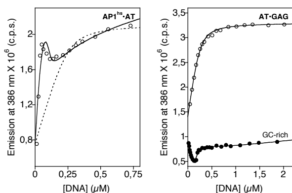
Figure 4. Left: Fluorescence emission titration of a 0.25 \mu\text{M} solution of GCN4-bb with a dsDNA containing the target sequence ( API hs •AT ) in Tris-HCl buffer 20 mM pH 7.5, 100 mM NaCl. Solid line represents a nonlinear fit to a mixed model considering a 1:1 complex and competitive species resulting from non-specific binding; dashed line represents the best fit to a simple 1:1 binding mode, discarding points 2 to 9 in the titration. Right: Titration of a 0.5 \mu\text{M} solution of GAGA-bb with a DNA containing the composite recognition site ( AT•GAG ) in Tris-HCl buffer 20 mM pH 7.5, 100 mM NaCl. Solid line represents the nonlinear fit to a 1:1 binding mode for AT•GAG , and a mixed mode including competitive nonspecific binding for the GC-rich oligonucleotide.
