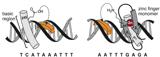
Figure 2. Left: schematic representation of the simultaneous interaction of the GCN4 basic region peptide (gray cylinder) and the bisbenzamide (orange block), indicating the Glu245 residue selected for conjugation. Right: representation of a simultaneous interaction of the DNA binding domain of the GAGA transcription factor fragment in the major groove, and the bisbenzamide in the minor groove. In this case Lys44 is selected as an appropriate conjugation position. The models used to design the synthetic targets were based on the reported structures of the DNA binding complexes of the GCN4 and GAGA transcription factors, 13 and that of pentamidine, 14 as described in earlier reports of distamycin hybrids. 7
