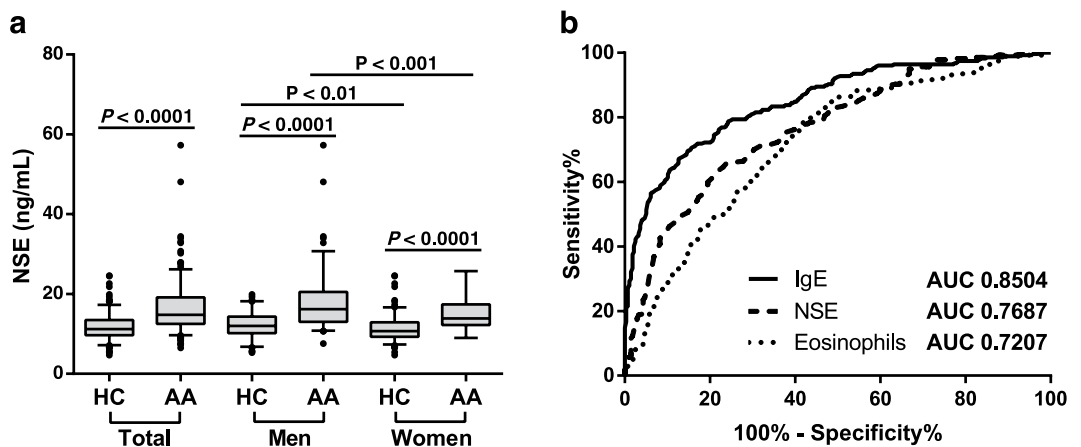
Figure 1. Analysis of NSE values in serum from AA and HC. (a) NSE levels in allergic asthmatics (AA) and healthy controls (HC) segregated by gender. Numbers on the graphs represent P -values (Mann-Whitney U test). (b) ROC curves for IgE, NSE and peripheral blood eosinophils. AUC values are shown for each parameter.
