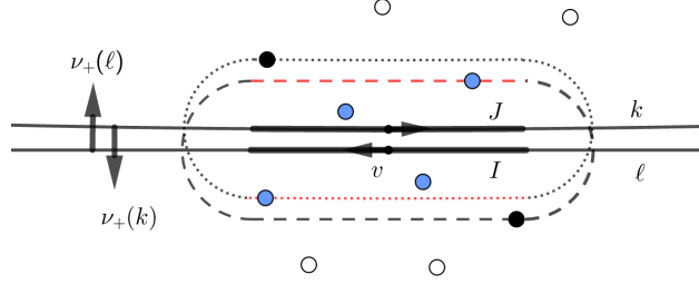
FIGURE 6. Approximation of S_\ell^+ by S_k^+ : The vectors \nu_+(\ell) and \nu_+(k) represent the orientations of the normal bundles of \ell and k , respectively. Two circles with dotted lines represent the boundary of the \rho -neighbourhoods of I and J , respectively. The dots represent points in \Gamma x . The blue dots belong to both E_\ell^+ and E_k^+ . But the black dots do not because they belong to the negative side of the boundary of E_\ell or E_k , respectively.
