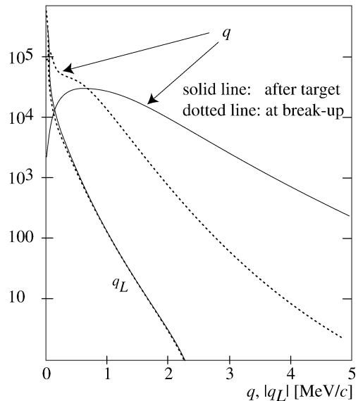
Fig. 1. Relative momentum distributions ( q , q_L ) for atomic \pi^+\pi^- pairs at the point of break-up and at the exit of the target. Note that q_L is almost not affected by multiple scattering in the target.
